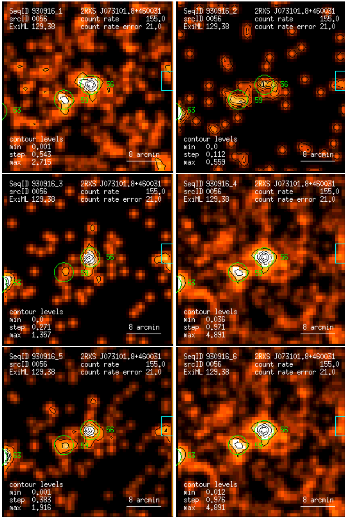
Figure 56: RASS 930916: detection 0056: band rate images, Gaussian filter: (1) PSPC channels 11 – 41, (2) 52 – 90, (3) 91 – 201, (4) 11 – 235, (5) 52 – 201, (6) 11 – 201. Broad band rates in counts/ks. Band rate contour levels in counts/ks/arcmin 2 .
