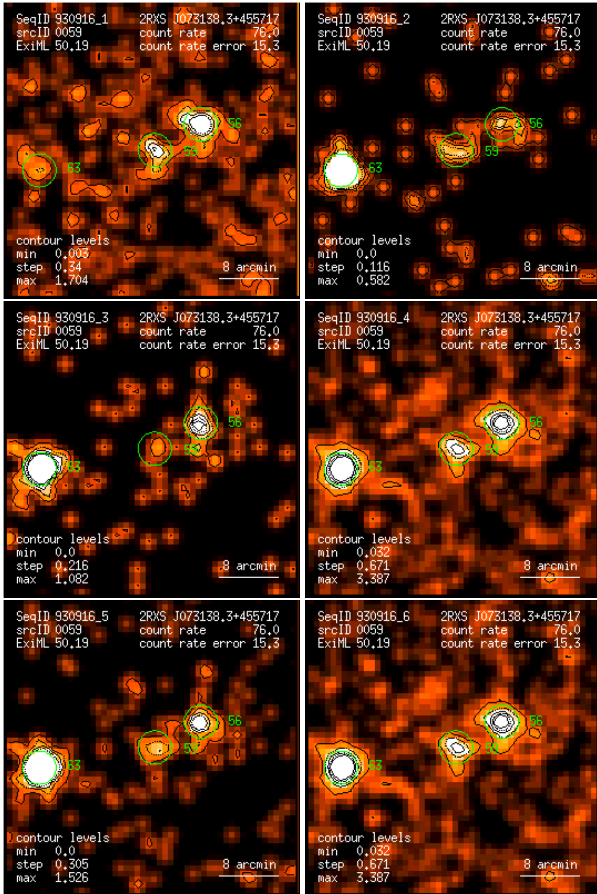
Figure 59: RASS 930916: detection 0059: band rate images, Gaussian filter: (1) PSPC channels 11 – 41, (2) 52 – 90, (3) 91 – 201, (4) 11 – 235, (5) 52 – 201, (6) 11 – 201. Broad band rates in counts/ks. Band rate contour levels in counts/ks/arcmin 2 .
