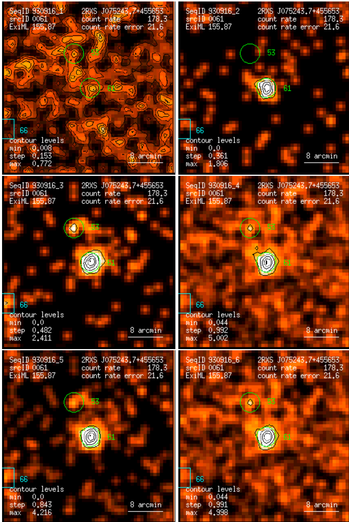
Figure 61: RASS 930916: detection 0061: band rate images, Gaussian filter: (1) PSPC channels 11 – 41, (2) 52 – 90, (3) 91 – 201, (4) 11 – 235, (5) 52 – 201, (6) 11 – 201. Broad band rates in counts/ks. Band rate contour levels in counts/ks/arcmin 2 .
