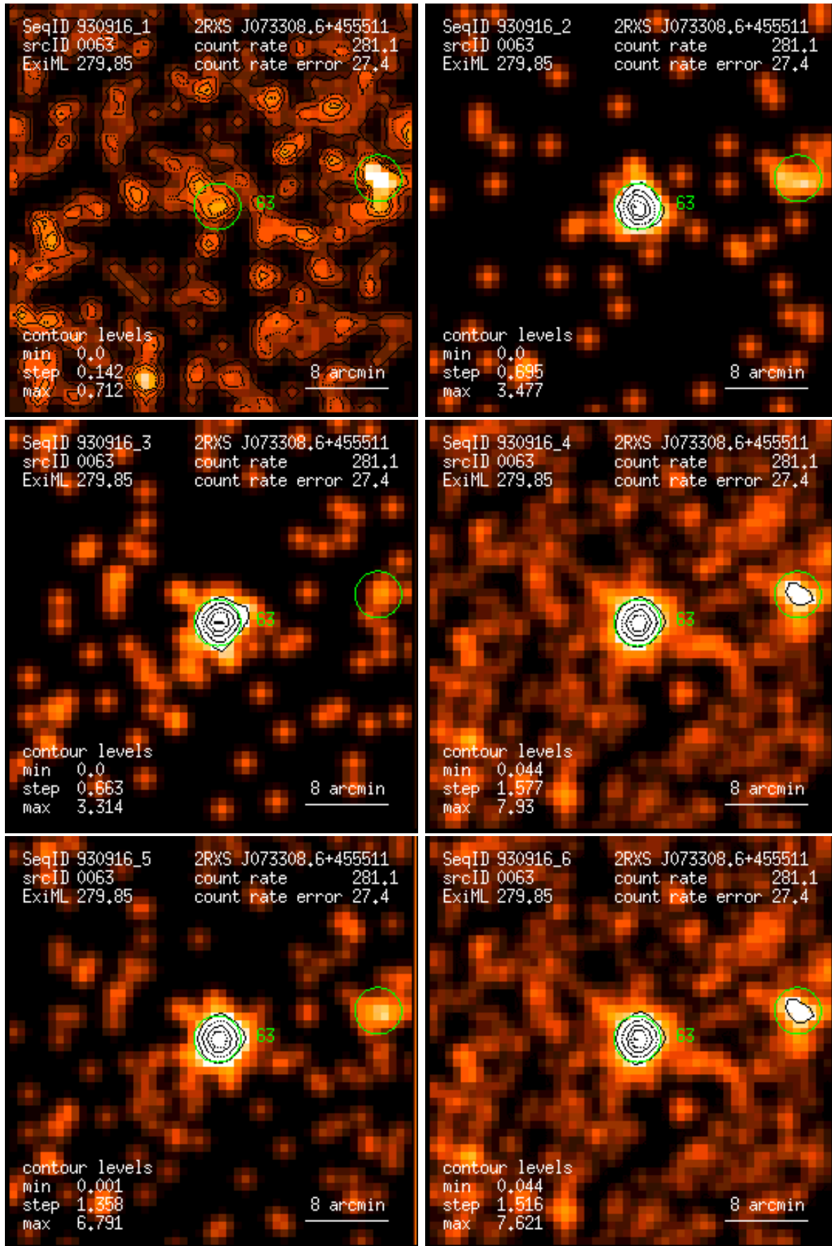
Figure 63: RASS 930916: detection 0063: band rate images, Gaussian filter: (1) PSPC channels 11 – 41, (2) 52 – 90, (3) 91 – 201, (4) 11 – 235, (5) 52 – 201, (6) 11 – 201. Broad band rates in counts/ks. Band rate contour levels in counts/ks/arcmin 2 .
