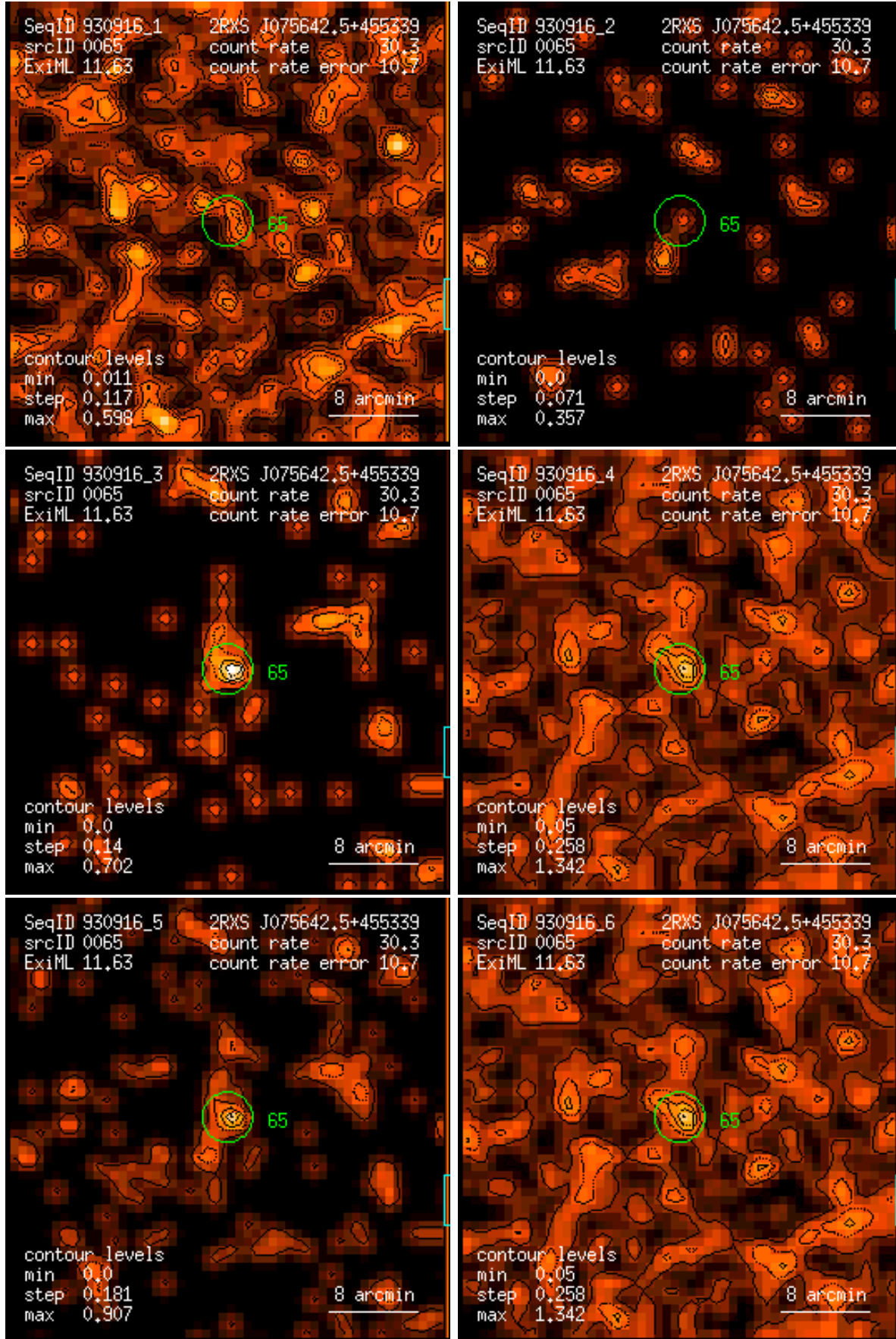
Figure 65: RASS 930916: detection 0065: band rate images, Gaussian filter: (1) PSPC channels 11 – 41, (2) 52 – 90, (3) 91 – 201, (4) 11 – 235, (5) 52 – 201, (6) 11 – 201. Broad band rates in counts/ks. Band rate contour levels in counts/ks/arcmin 2 .
