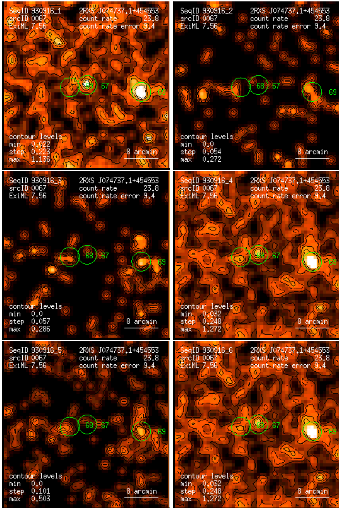
Figure 67: RASS 930916: detection 0067: band rate images, Gaussian filter: (1) PSPC channels 11 – 41, (2) 52 – 90, (3) 91 – 201, (4) 11 – 235, (5) 52 – 201, (6) 11 – 201. Broad band rates in counts/ks. Band rate contour levels in counts/ks/arcmin 2 .
