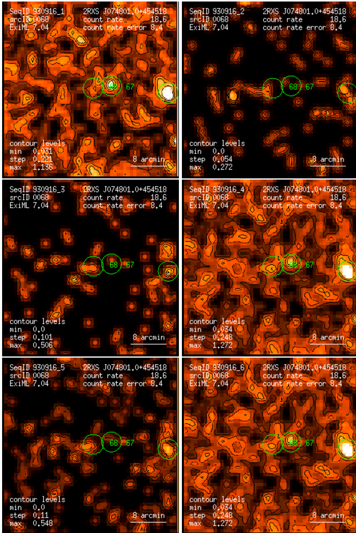
Figure 68: RASS 930916: detection 0068: band rate images, Gaussian filter: (1) PSPC channels 11 – 41, (2) 52 – 90, (3) 91 – 201, (4) 11 – 235, (5) 52 – 201, (6) 11 – 201. Broad band rates in counts/ks. Band rate contour levels in counts/ks/arcmin 2 .
