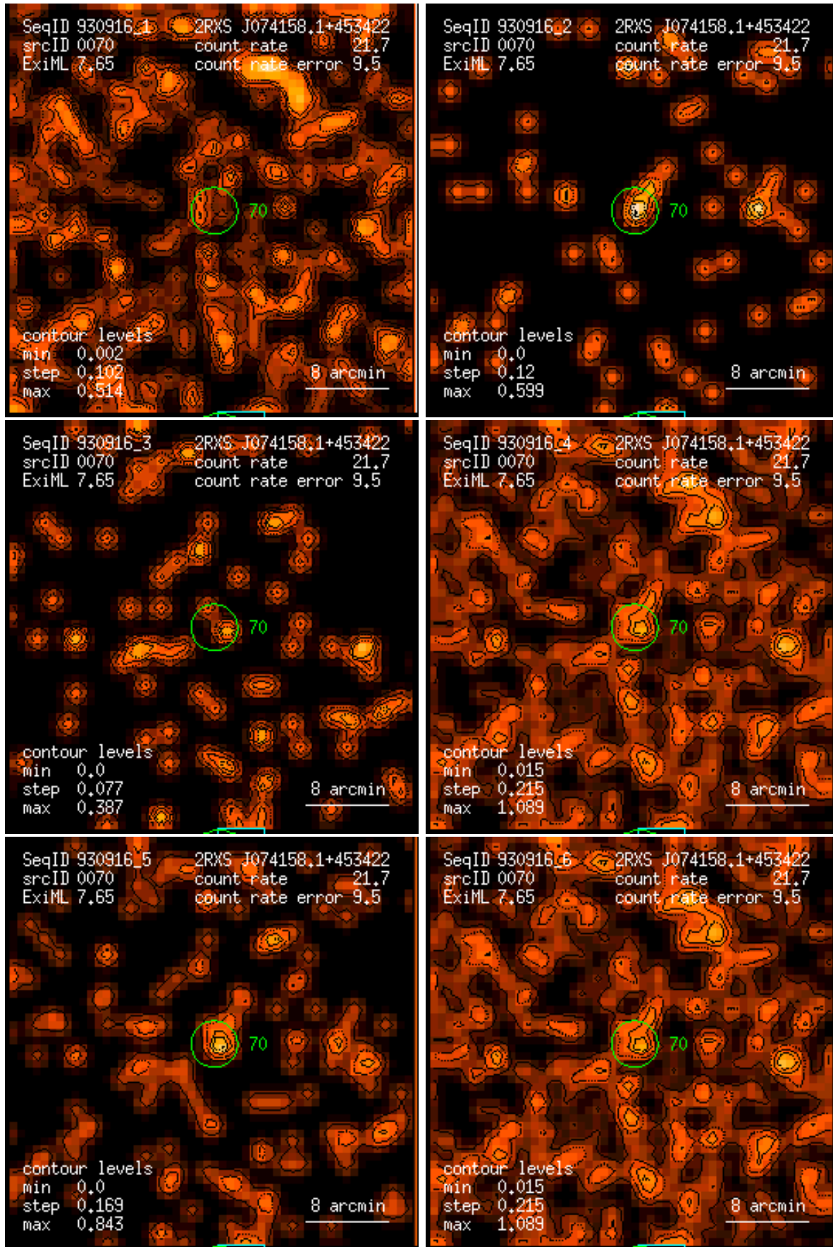
Figure 70: RASS 930916: detection 0070: band rate images, Gaussian filter: (1) PSPC channels 11 – 41, (2) 52 – 90, (3) 91 – 201, (4) 11 – 235, (5) 52 – 201, (6) 11 – 201. Broad band rates in counts/ks. Band rate contour levels in counts/ks/arcmin 2 .
