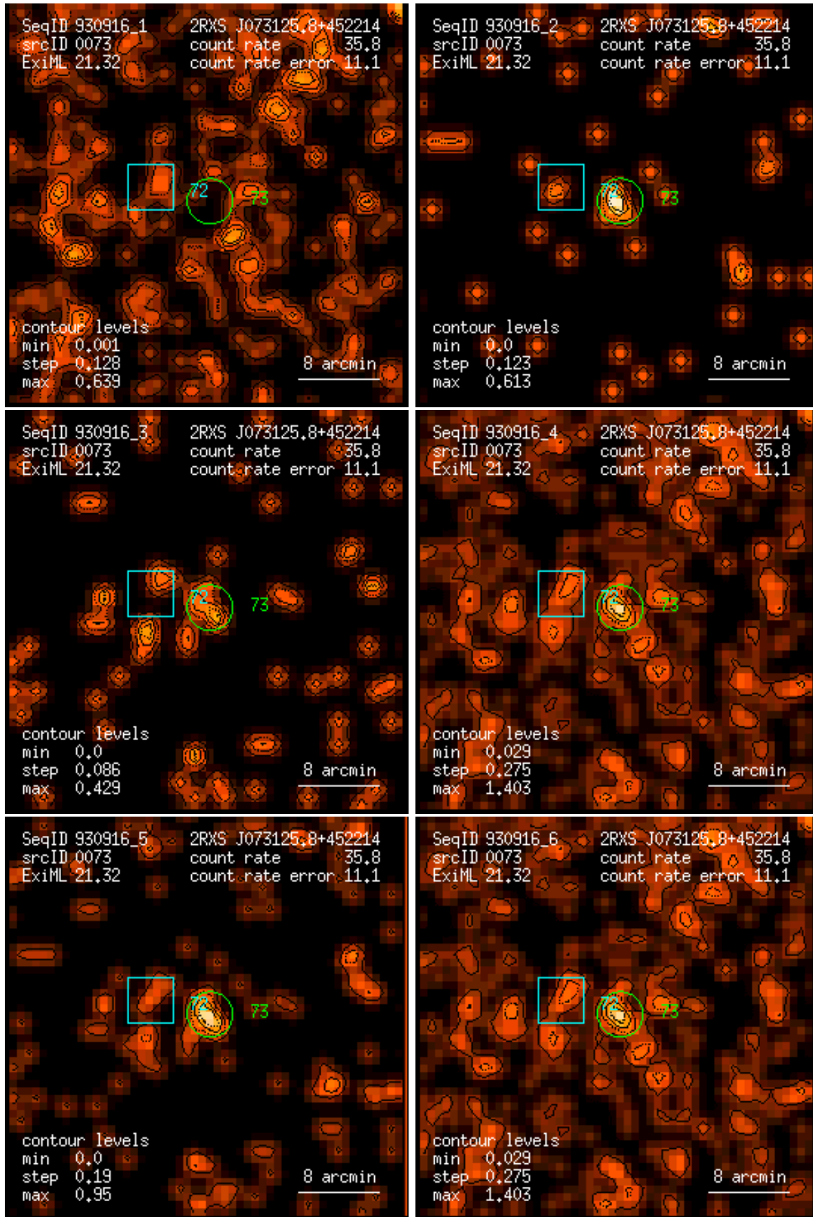
Figure 73: RASS 930916: detection 0073: band rate images, Gaussian filter: (1) PSPC channels 11 – 41, (2) 52 – 90, (3) 91 – 201, (4) 11 – 235, (5) 52 – 201, (6) 11 – 201. Broad band rates in counts/ks. Band rate contour levels in counts/ks/arcmin 2 .
