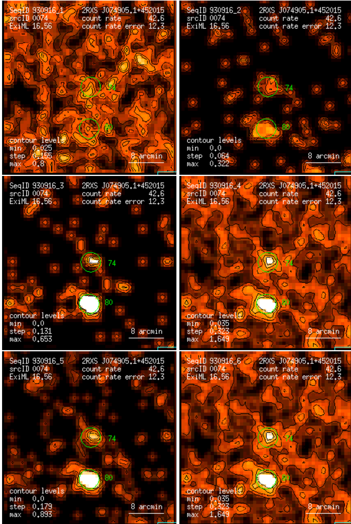
Figure 74: RASS 930916: detection 0074: band rate images, Gaussian filter: (1) PSPC channels 11 – 41, (2) 52 – 90, (3) 91 – 201, (4) 11 – 235, (5) 52 – 201, (6) 11 – 201. Broad band rates in counts/ks. Band rate contour levels in counts/ks/arcmin 2 .
