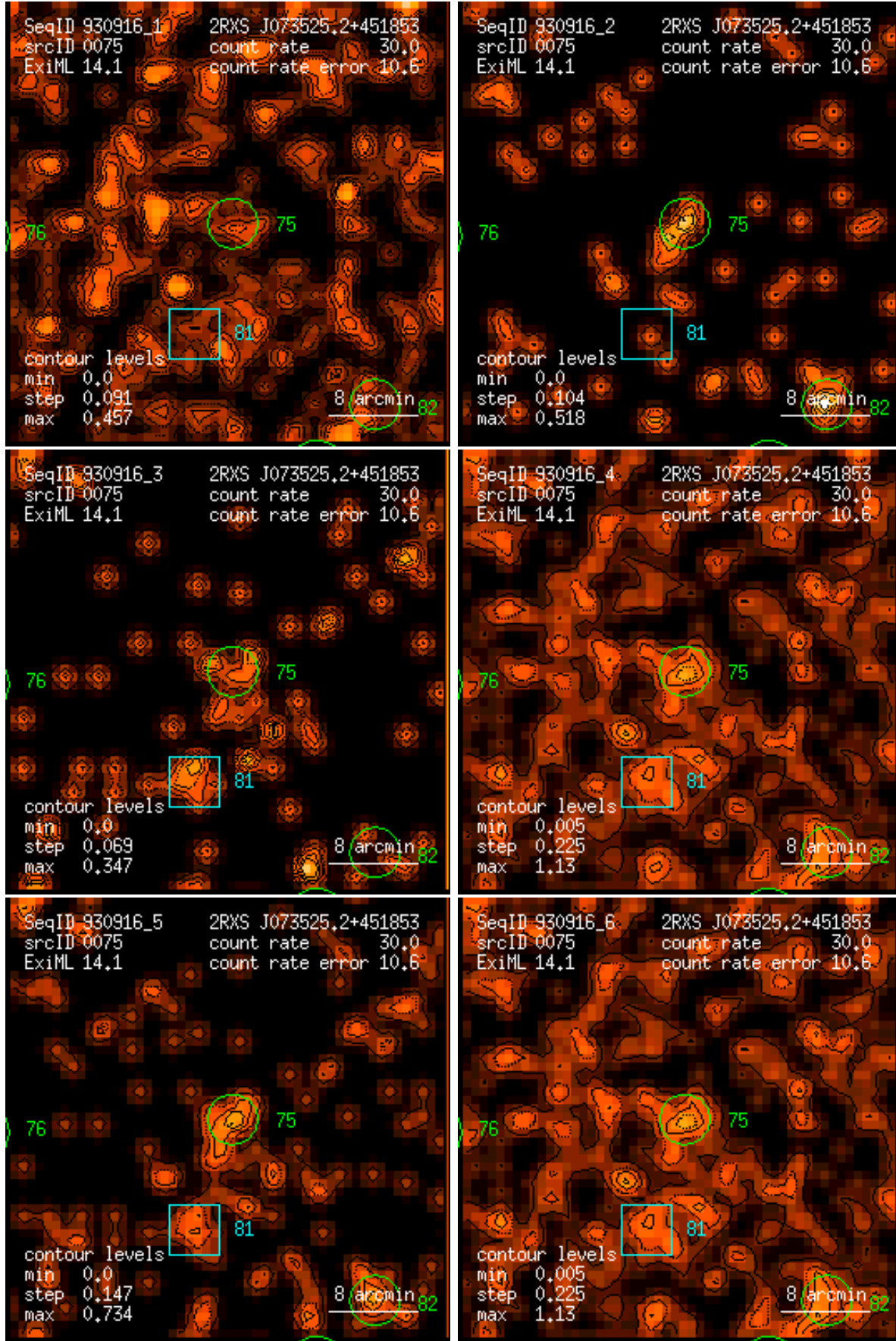
Figure 75: RASS 930916: detection 0075: band rate images, Gaussian filter: (1) PSPC channels 11 – 41, (2) 52 – 90, (3) 91 – 201, (4) 11 – 235, (5) 52 – 201, (6) 11 – 201. Broad band rates in counts/ks. Band rate contour levels in counts/ks/arcmin 2 .
