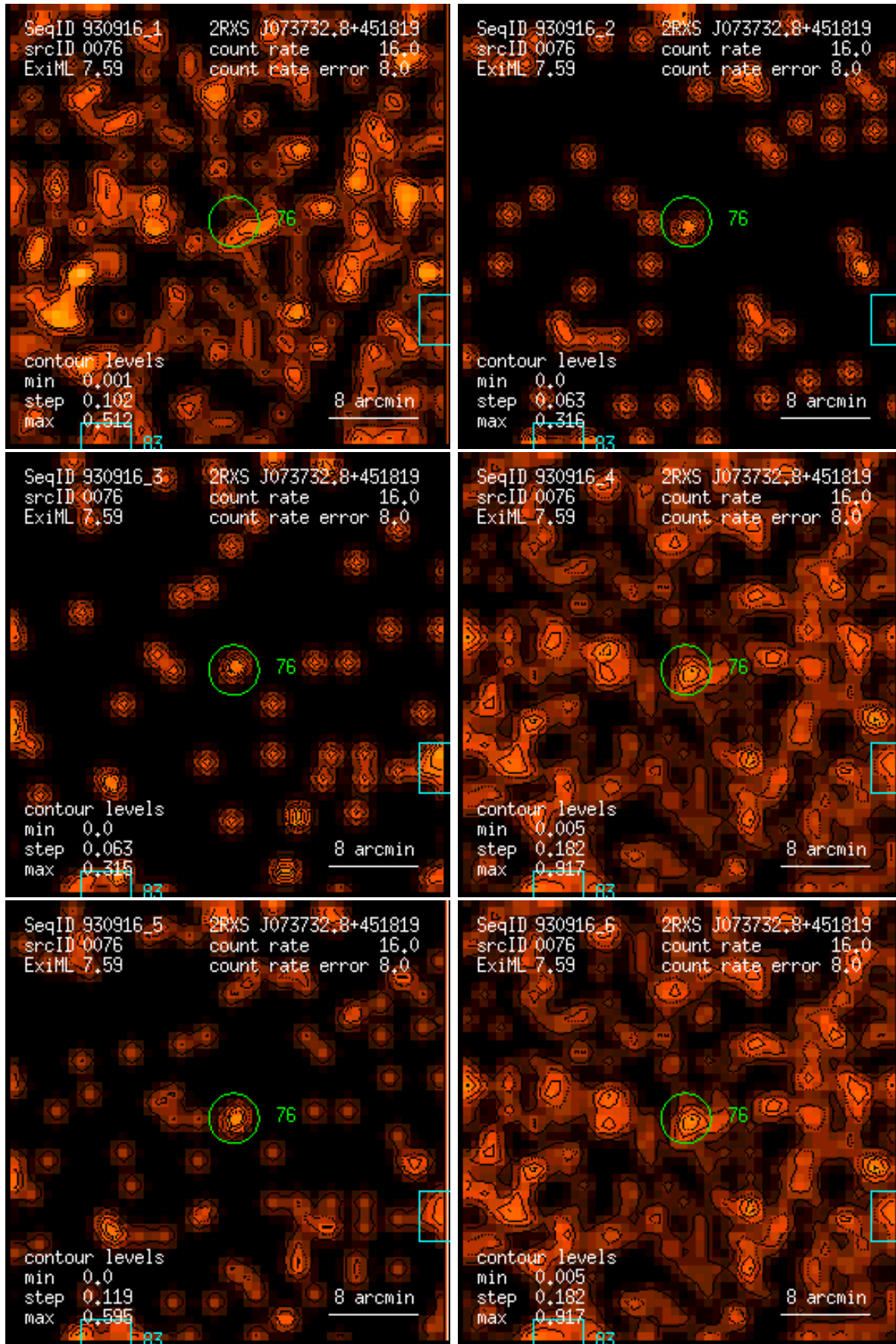
Figure 76: RASS 930916: detection 0076: band rate images, Gaussian filter: (1) PSPC channels 11 – 41, (2) 52 – 90, (3) 91 – 201, (4) 11 – 235, (5) 52 – 201, (6) 11 – 201. Broad band rates in counts/ks. Band rate contour levels in counts/ks/arcmin 2 .
