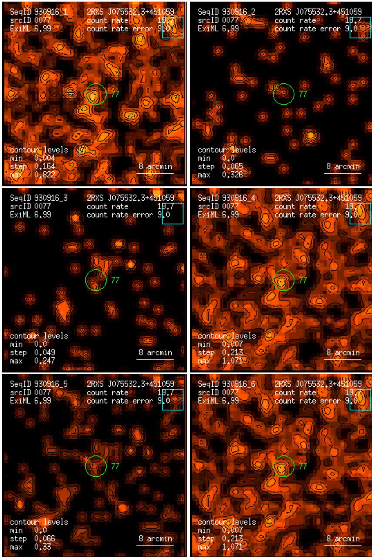
Figure 77: RASS 930916: detection 0077: band rate images, Gaussian filter: (1) PSPC channels 11 – 41, (2) 52 – 90, (3) 91 – 201, (4) 11 – 235, (5) 52 – 201, (6) 11 – 201. Broad band rates in counts/ks. Band rate contour levels in counts/ks/arcmin 2 .
