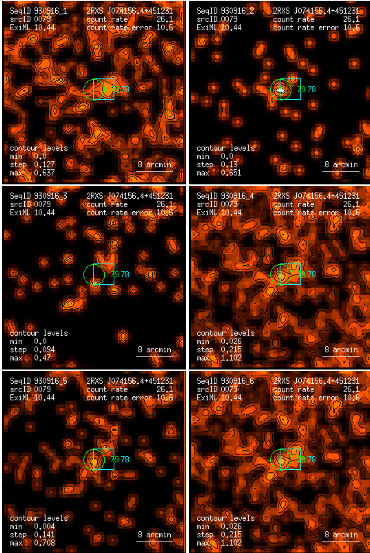
Figure 79: RASS 930916: detection 0079: band rate images, Gaussian filter: (1) PSPC channels 11 – 41, (2) 52 – 90, (3) 91 – 201, (4) 11 – 235, (5) 52 – 201, (6) 11 – 201. Broad band rates in counts/ks. Band rate contour levels in counts/ks/arcmin 2 .
