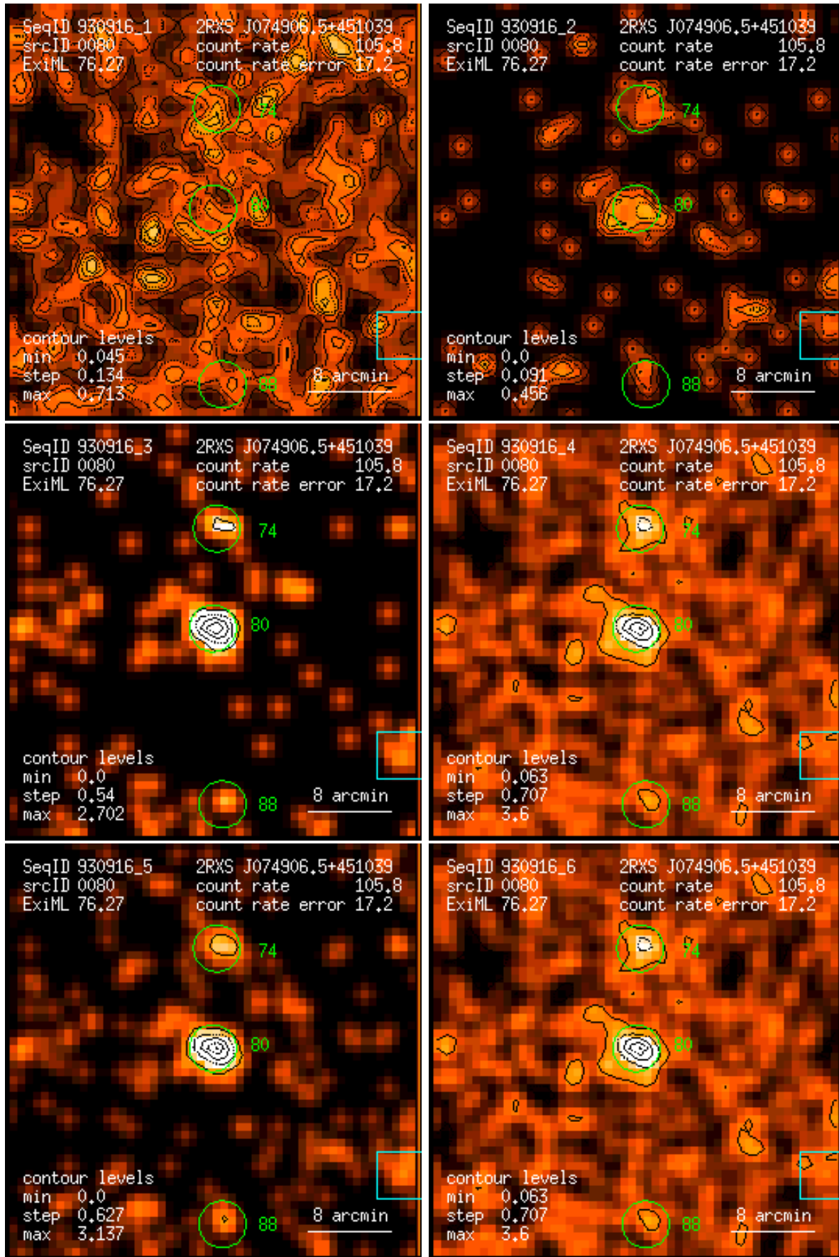
Figure 80: RASS 930916: detection 0080: band rate images, Gaussian filter: (1) PSPC channels 11 – 41, (2) 52 – 90, (3) 91 – 201, (4) 11 – 235, (5) 52 – 201, (6) 11 – 201. Broad band rates in counts/ks. Band rate contour levels in counts/ks/arcmin 2 .
