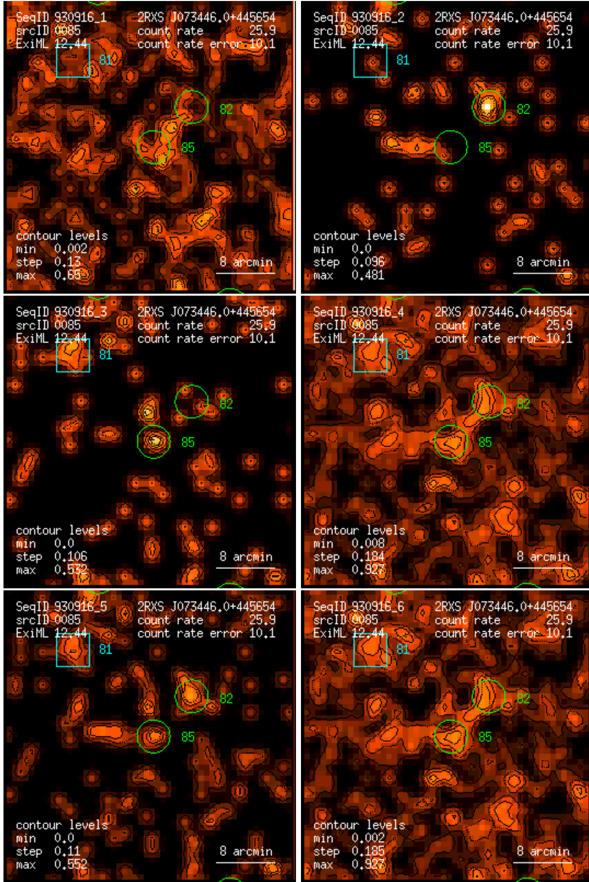
Figure 85: RASS 930916: detection 0085: band rate images, Gaussian filter: (1) PSPC channels 11 – 41, (2) 52 – 90, (3) 91 – 201, (4) 11 – 235, (5) 52 – 201, (6) 11 – 201. Broad band rates in counts/ks. Band rate contour levels in counts/ks/arcmin 2 .
