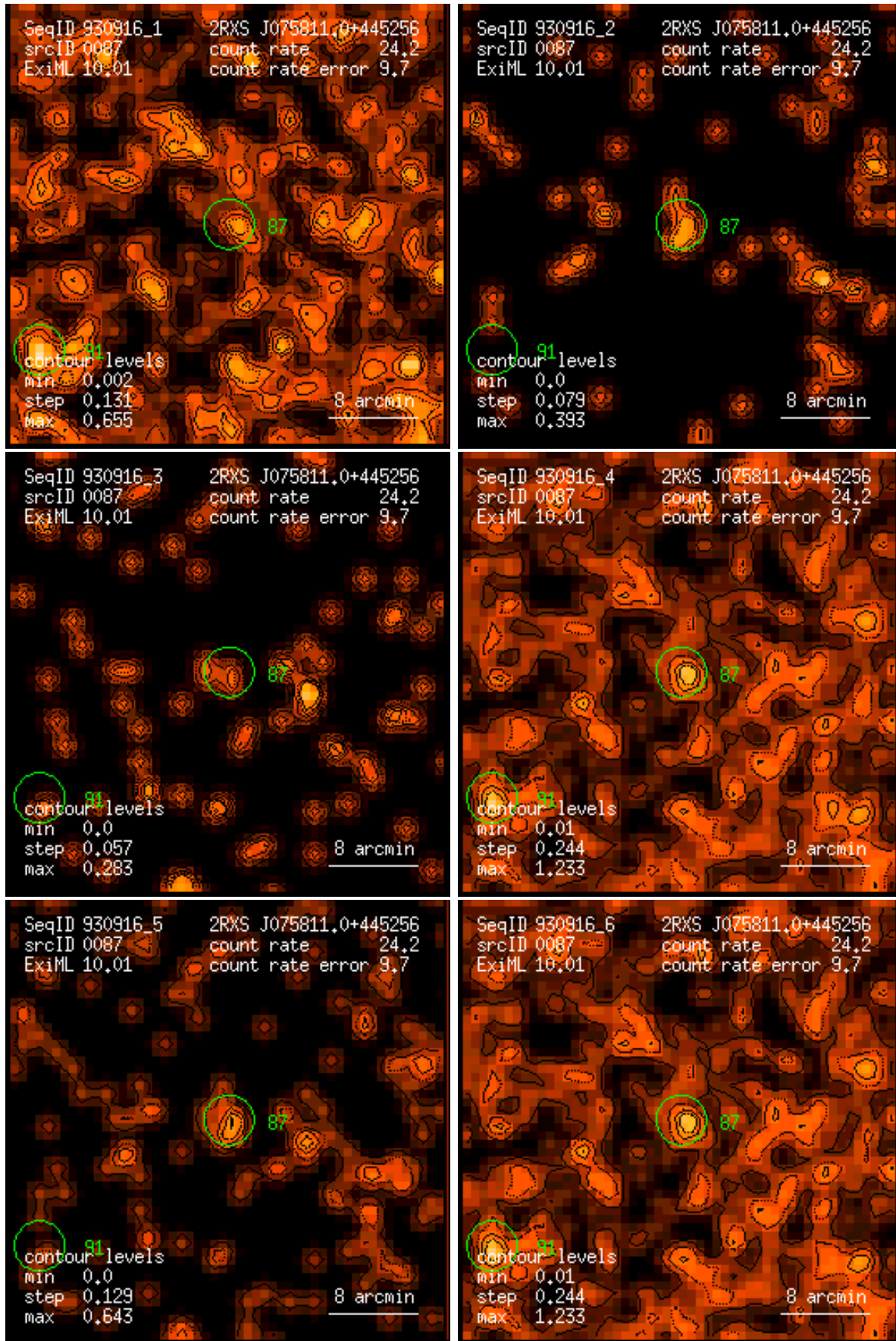
Figure 87: RASS 930916: detection 0087: band rate images, Gaussian filter: (1) PSPC channels 11 – 41, (2) 52 – 90, (3) 91 – 201, (4) 11 – 235, (5) 52 – 201, (6) 11 – 201. Broad band rates in counts/ks. Band rate contour levels in counts/ks/arcmin 2 .
