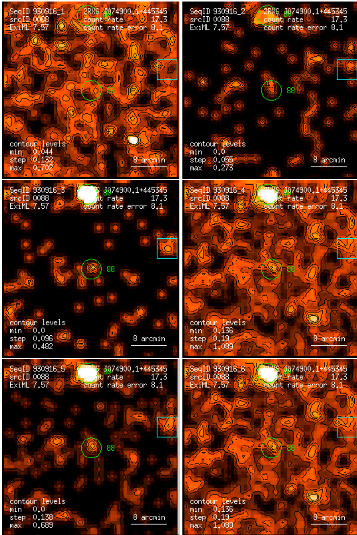
Figure 88: RASS 930916: detection 0088: band rate images, Gaussian filter: (1) PSPC channels 11 – 41, (2) 52 – 90, (3) 91 – 201, (4) 11 – 235, (5) 52 – 201, (6) 11 – 201. Broad band rates in counts/ks. Band rate contour levels in counts/ks/arcmin 2 .
