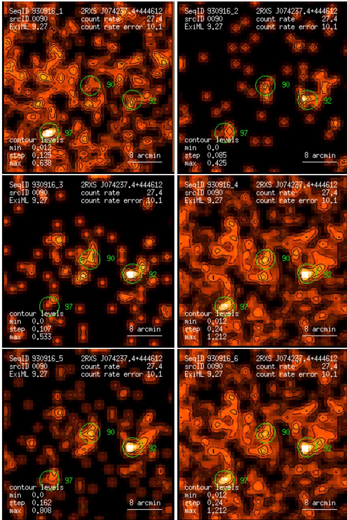
Figure 90: RASS 930916: detection 0090: band rate images, Gaussian filter: (1) PSPC channels 11 – 41, (2) 52 – 90, (3) 91 – 201, (4) 11 – 235, (5) 52 – 201, (6) 11 – 201. Broad band rates in counts/ks. Band rate contour levels in counts/ks/arcmin 2 .
