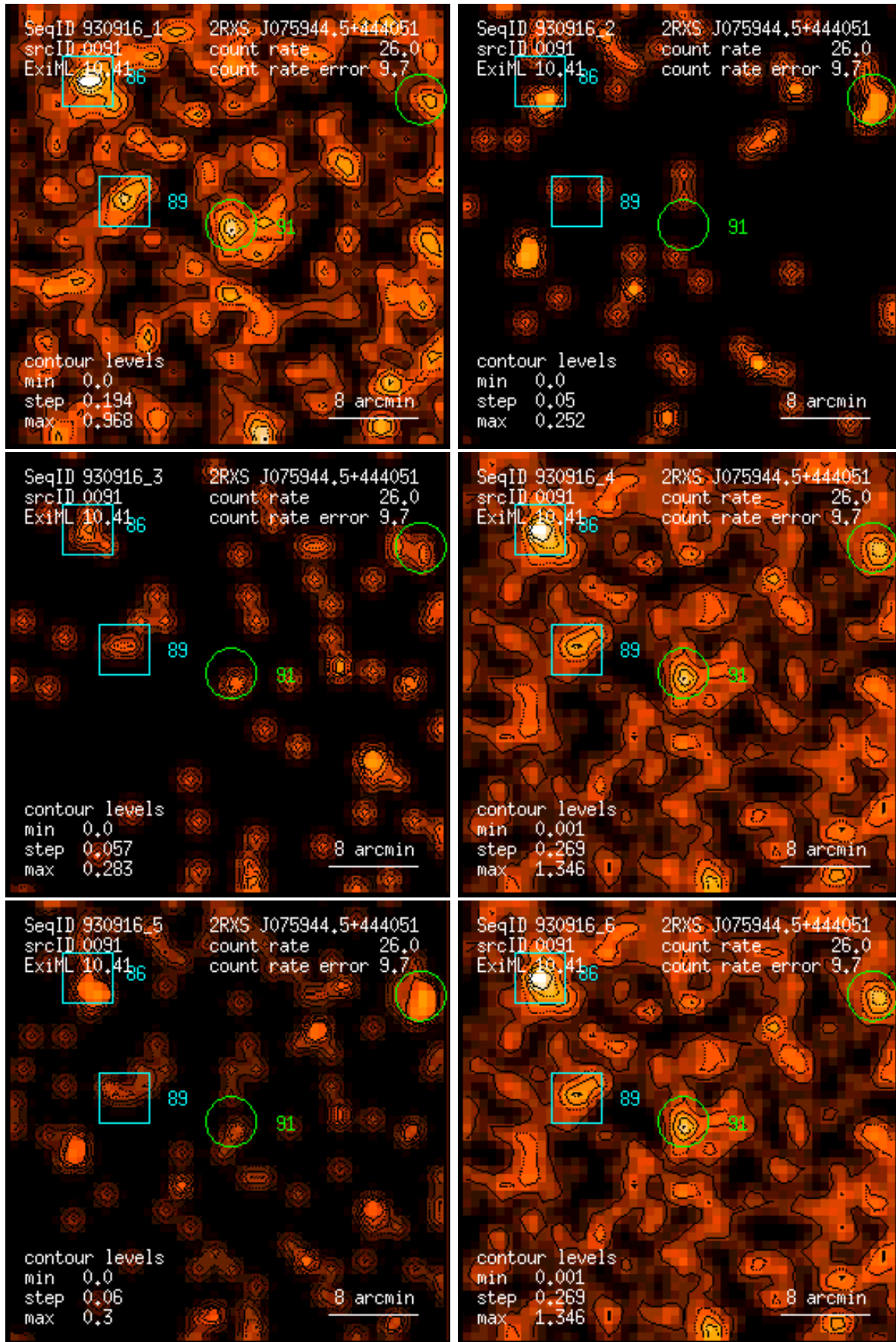
Figure 91: RASS 930916: detection 0091: band rate images, Gaussian filter: (1) PSPC channels 11 – 41, (2) 52 – 90, (3) 91 – 201, (4) 11 – 235, (5) 52 – 201, (6) 11 – 201. Broad band rates in counts/ks. Band rate contour levels in counts/ks/arcmin 2 .
