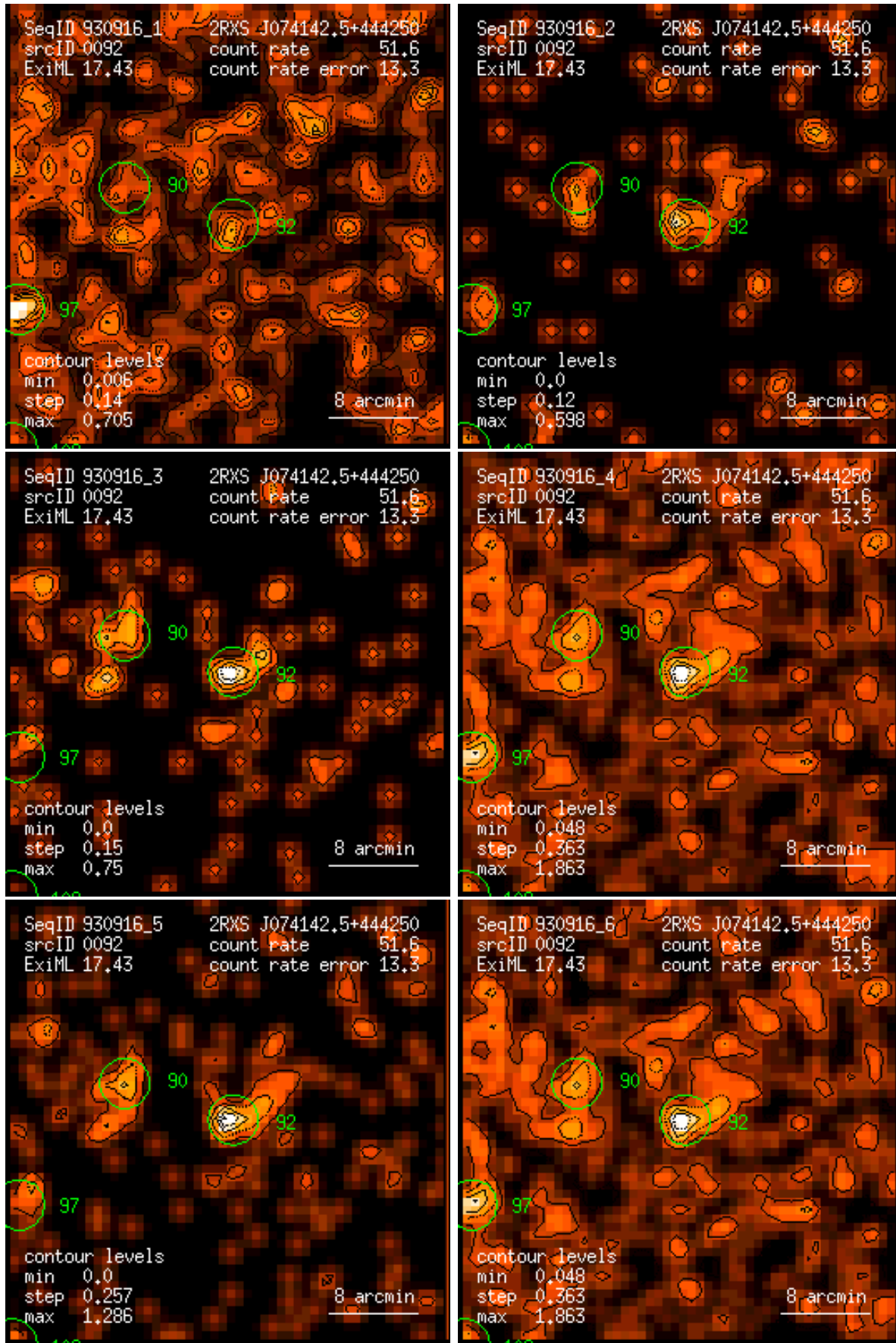
Figure 92: RASS 930916: detection 0092: band rate images, Gaussian filter: (1) PSPC channels 11 – 41, (2) 52 – 90, (3) 91 – 201, (4) 11 – 235, (5) 52 – 201, (6) 11 – 201. Broad band rates in counts/ks. Band rate contour levels in counts/ks/arcmin 2 .
