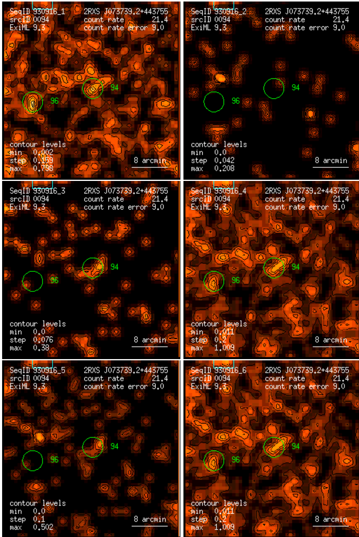
Figure 94: RASS 930916: detection 0094: band rate images, Gaussian filter: (1) PSPC channels 11 – 41, (2) 52 – 90, (3) 91 – 201, (4) 11 – 235, (5) 52 – 201, (6) 11 – 201. Broad band rates in counts/ks. Band rate contour levels in counts/ks/arcmin 2 .
