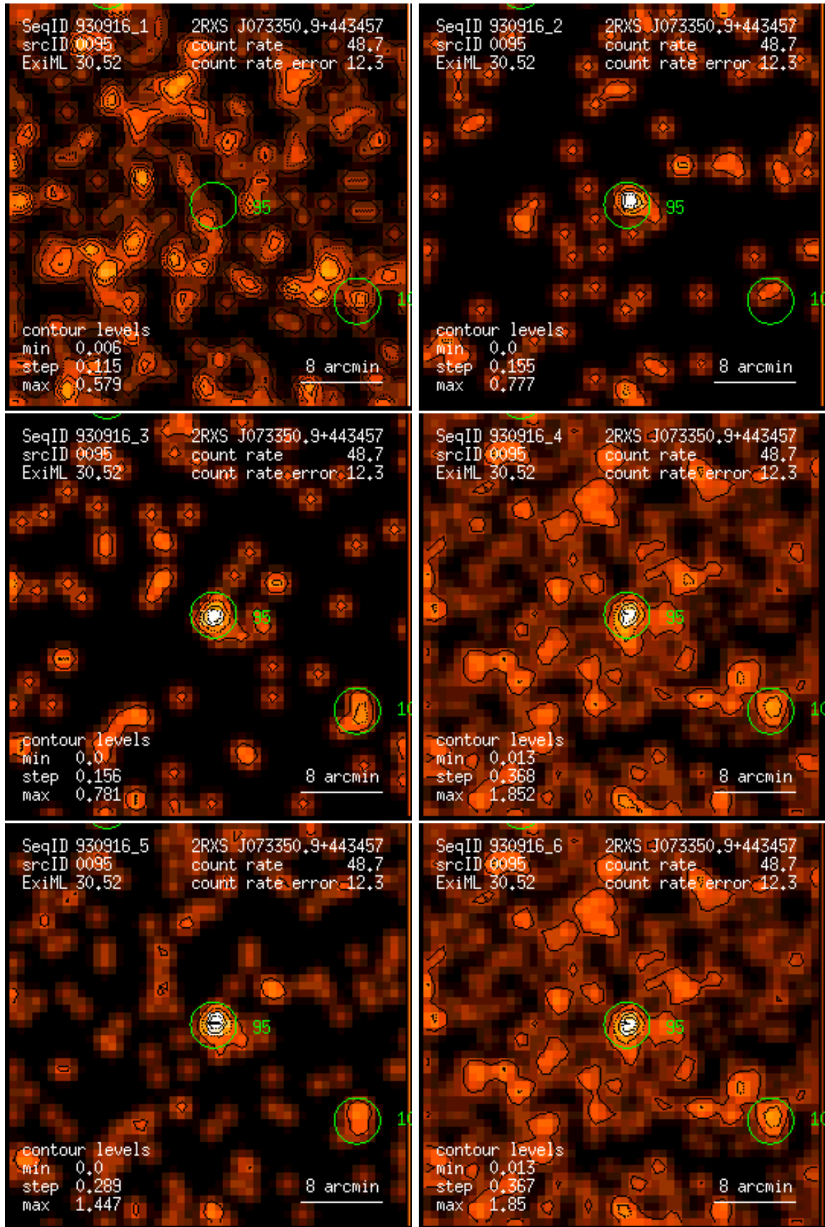
Figure 95: RASS 930916: detection 0095: band rate images, Gaussian filter: (1) PSPC channels 11 – 41, (2) 52 – 90, (3) 91 – 201, (4) 11 – 235, (5) 52 – 201, (6) 11 – 201. Broad band rates in counts/ks. Band rate contour levels in counts/ks/arcmin 2 .
