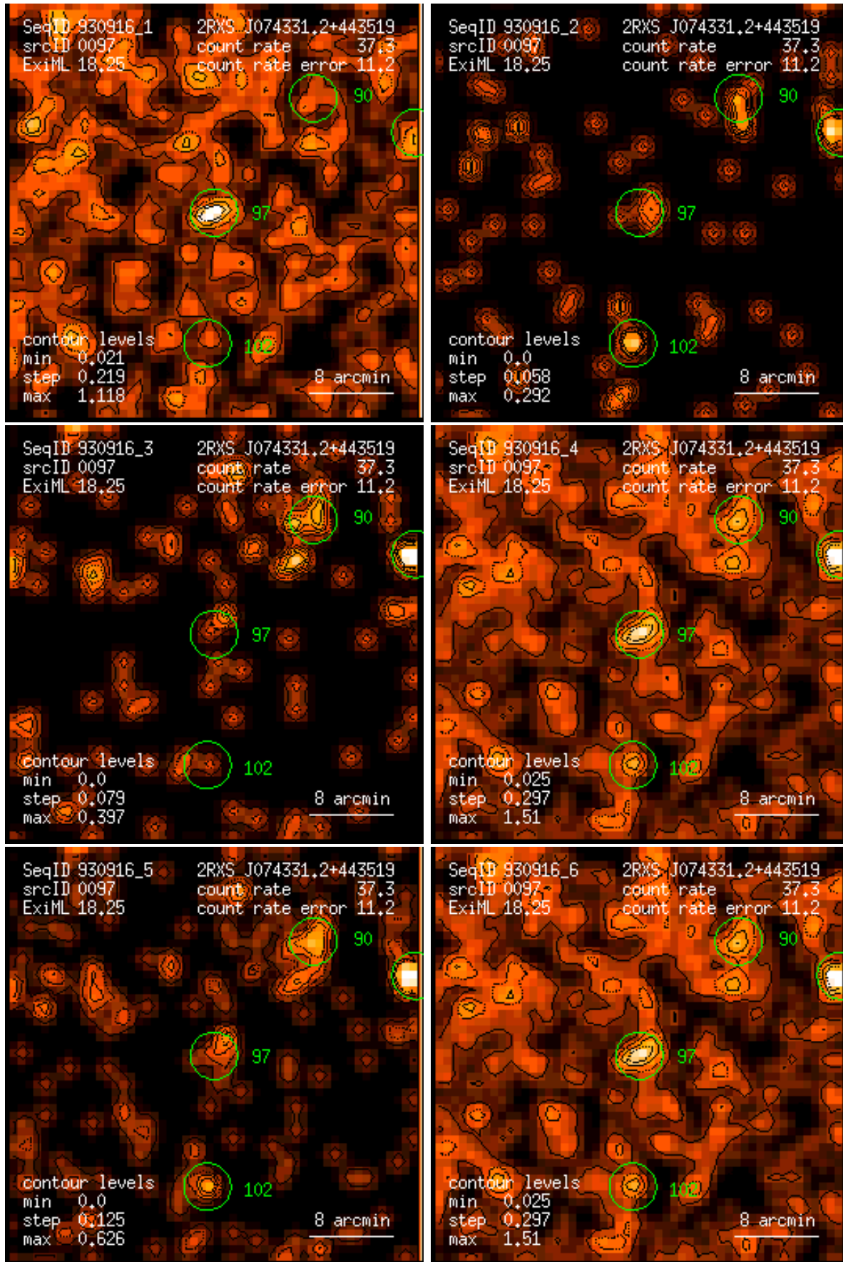
Figure 97: RASS 930916: detection 0097: band rate images, Gaussian filter: (1) PSPC channels 11 – 41, (2) 52 – 90, (3) 91 – 201, (4) 11 – 235, (5) 52 – 201, (6) 11 – 201. Broad band rates in counts/ks. Band rate contour levels in counts/ks/arcmin 2 .
