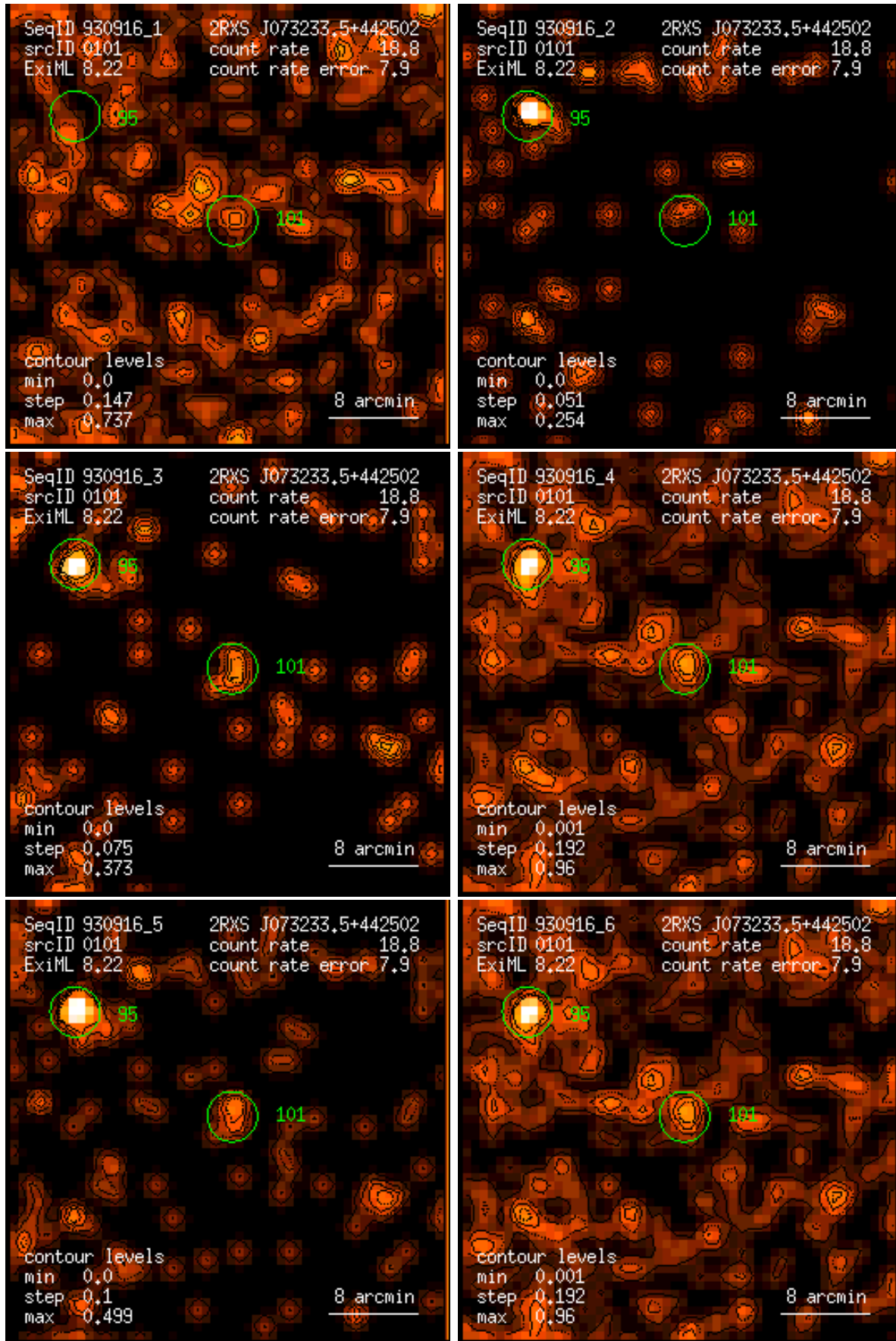
Figure 101: RASS 930916: detection 0101: band rate images, Gaussian filter: (1) PSPC channels 11 – 41, (2) 52 – 90, (3) 91 – 201, (4) 11 – 235, (5) 52 – 201, (6) 11 – 201. Broad band rates in counts/ks. Band rate contour levels in counts/ks/arcmin 2 .
