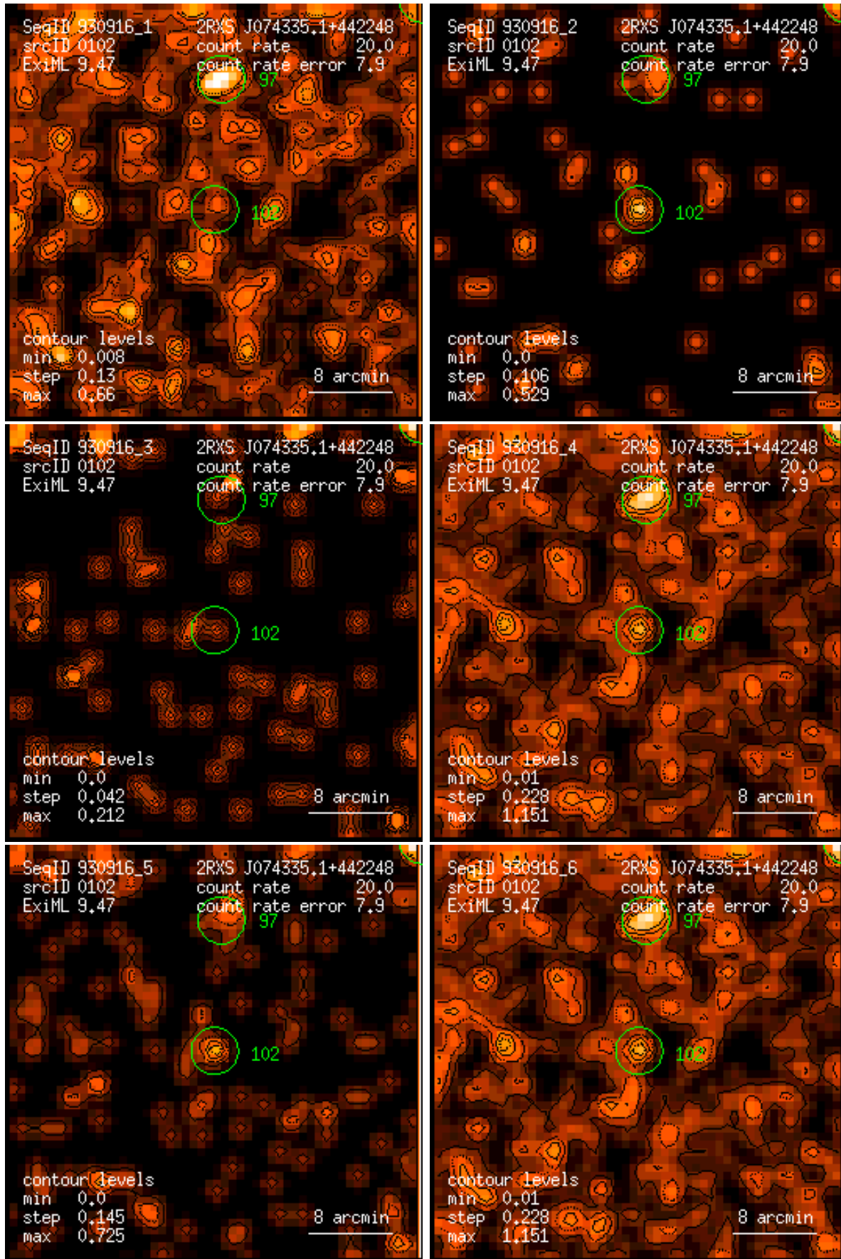
Figure 102: RASS 930916: detection 0102: band rate images, Gaussian filter: (1) PSPC channels 11 – 41, (2) 52 – 90, (3) 91 – 201, (4) 11 – 235, (5) 52 – 201, (6) 11 – 201. Broad band rates in counts/ks. Band rate contour levels in counts/ks/arcmin 2 .
