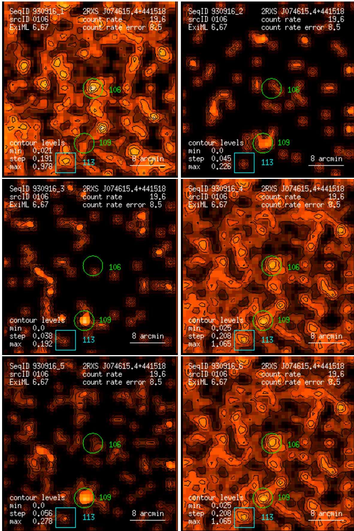
Figure 106: RASS 930916: detection 0106: band rate images, Gaussian filter: (1) PSPC channels 11 – 41, (2) 52 – 90, (3) 91 – 201, (4) 11 – 235, (5) 52 – 201, (6) 11 – 201. Broad band rates in counts/ks. Band rate contour levels in counts/ks/arcmin 2 .
