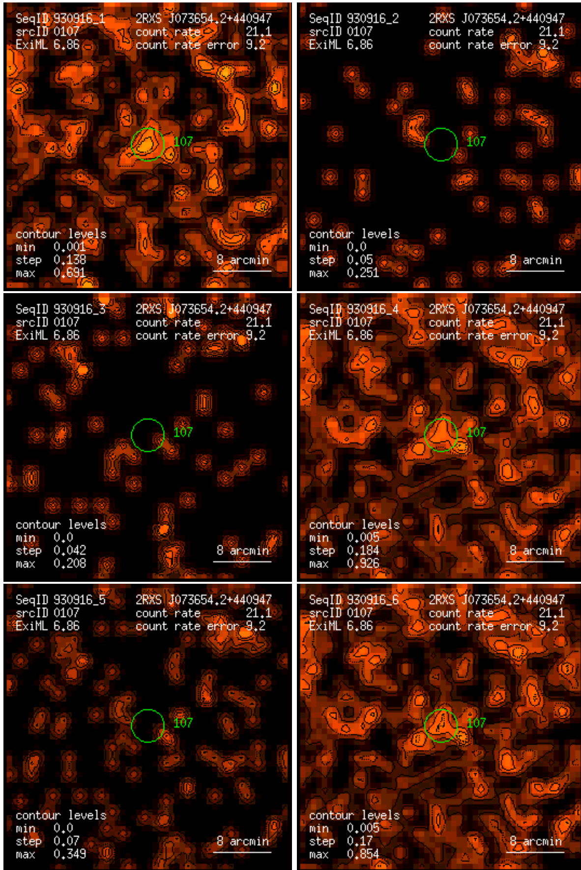
Figure 107: RASS 930916: detection 0107: band rate images, Gaussian filter: (1) PSPC channels 11 – 41, (2) 52 – 90, (3) 91 – 201, (4) 11 – 235, (5) 52 – 201, (6) 11 – 201. Broad band rates in counts/ks. Band rate contour levels in counts/ks/arcmin 2 .
