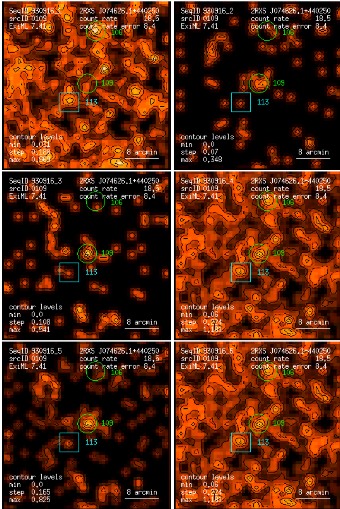
Figure 109: RASS 930916: detection 0109: band rate images, Gaussian filter: (1) PSPC channels 11 – 41, (2) 52 – 90, (3) 91 – 201, (4) 11 – 235, (5) 52 – 201, (6) 11 – 201. Broad band rates in counts/ks. Band rate contour levels in counts/ks/arcmin 2 .
