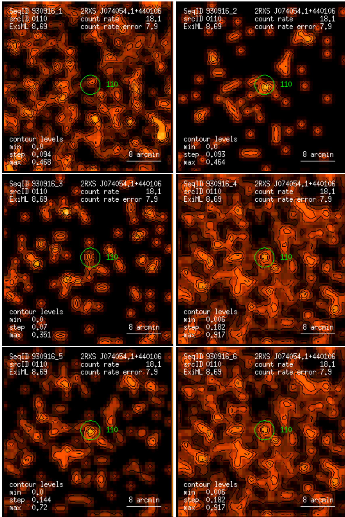
Figure 110: RASS 930916: detection 0110: band rate images, Gaussian filter: (1) PSPC channels 11 – 41, (2) 52 – 90, (3) 91 – 201, (4) 11 – 235, (5) 52 – 201, (6) 11 – 201. Broad band rates in counts/ks. Band rate contour levels in counts/ks/arcmin 2 .
