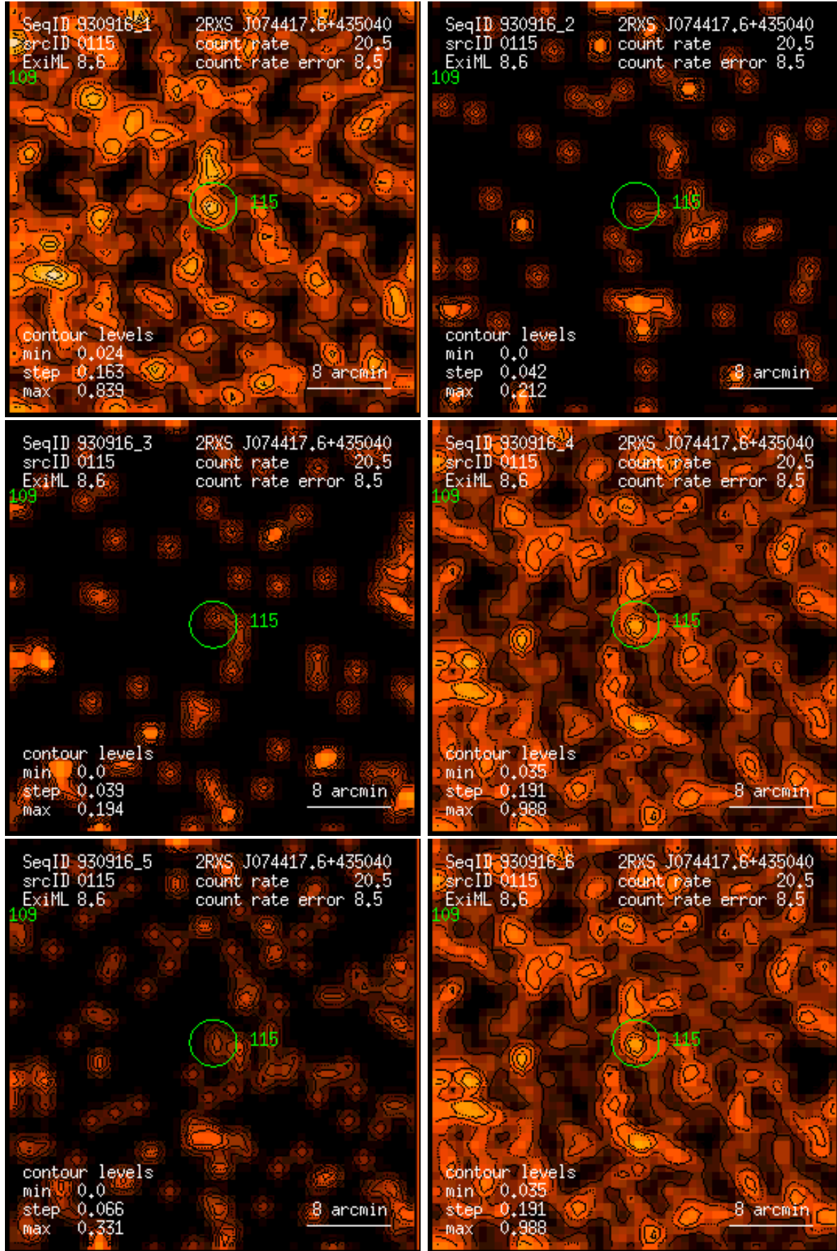
Figure 115: RASS 930916: detection 0115: band rate images, Gaussian filter: (1) PSPC channels 11 – 41, (2) 52 – 90, (3) 91 – 201, (4) 11 – 235, (5) 52 – 201, (6) 11 – 201. Broad band rates in counts/ks. Band rate contour levels in counts/ks/arcmin 2 .
