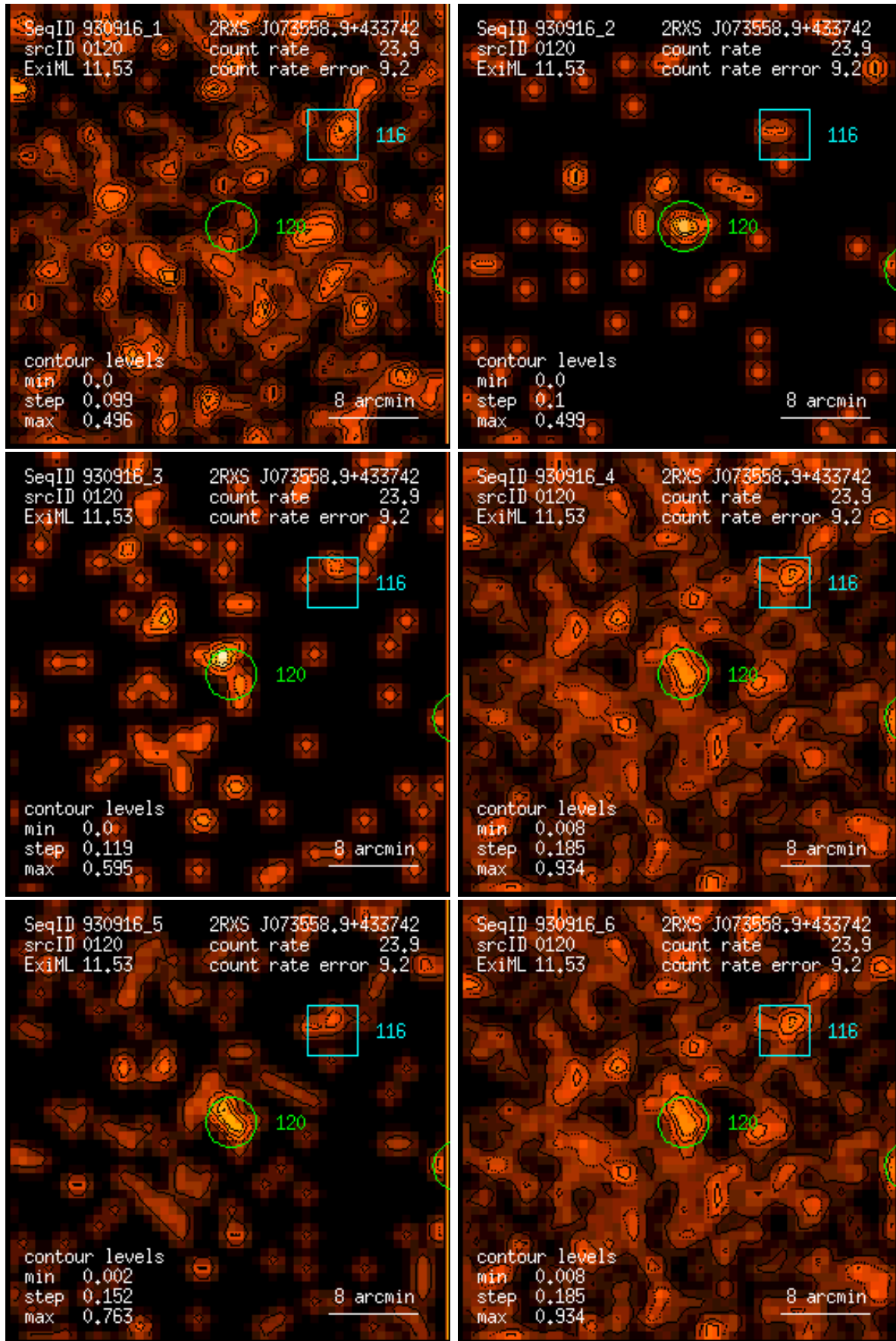
Figure 120: RASS 930916: detection 0120: band rate images, Gaussian filter: (1) PSPC channels 11 – 41, (2) 52 – 90, (3) 91 – 201, (4) 11 – 235, (5) 52 – 201, (6) 11 – 201. Broad band rates in counts/ks. Band rate contour levels in counts/ks/arcmin 2 .
