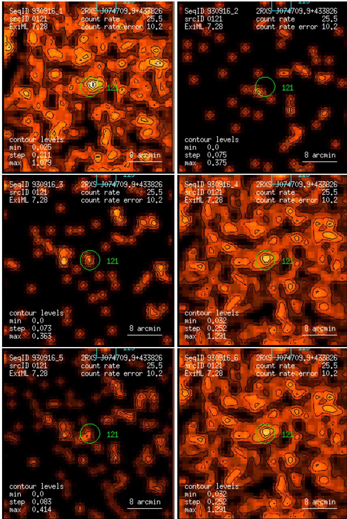
Figure 121: RASS 930916: detection 0121: band rate images, Gaussian filter: (1) PSPC channels 11 – 41, (2) 52 – 90, (3) 91 – 201, (4) 11 – 235, (5) 52 – 201, (6) 11 – 201. Broad band rates in counts/ks. Band rate contour levels in counts/ks/arcmin 2 .
