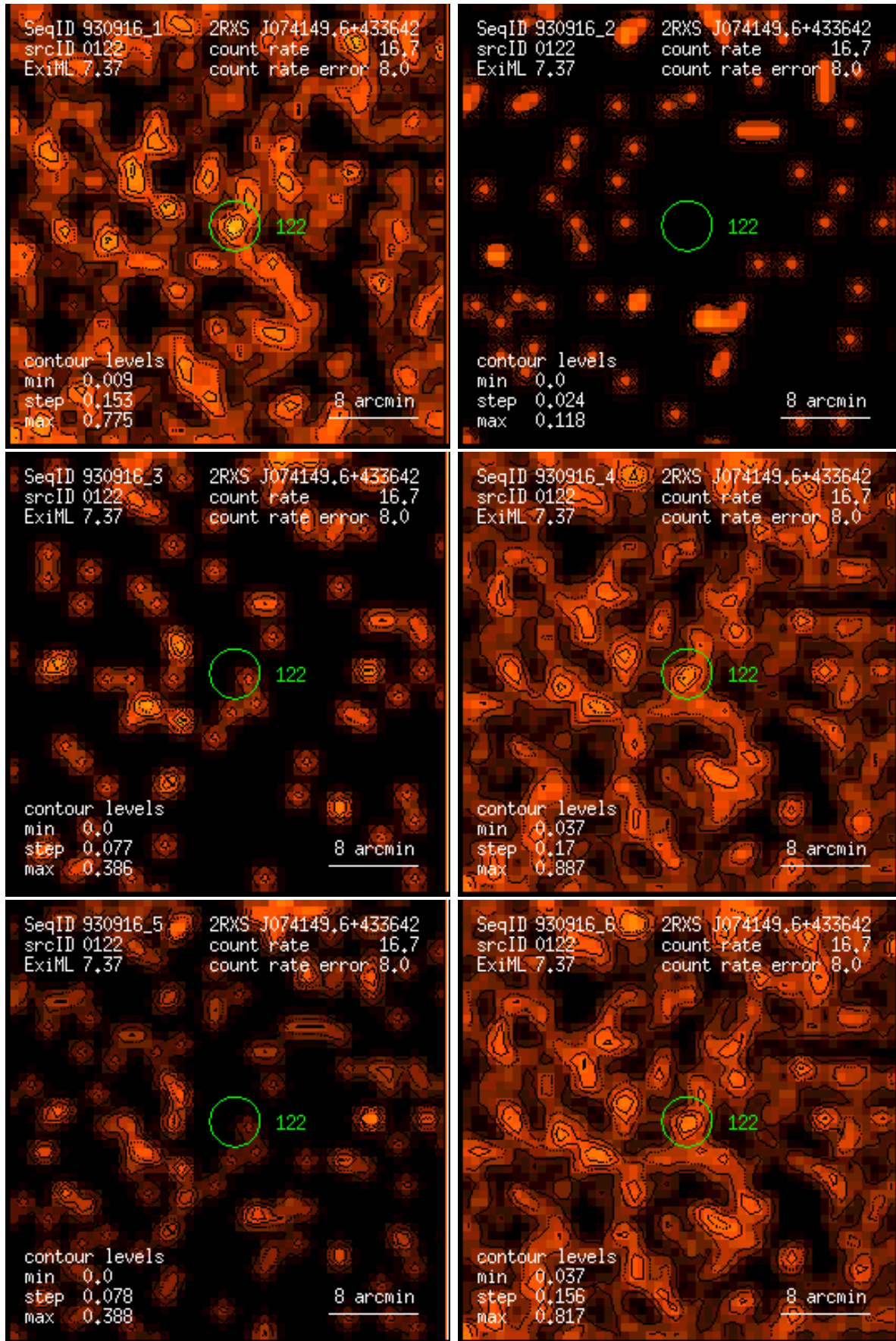
Figure 122: RASS 930916: detection 0122: band rate images, Gaussian filter: (1) PSPC channels 11 – 41, (2) 52 – 90, (3) 91 – 201, (4) 11 – 235, (5) 52 – 201, (6) 11 – 201. Broad band rates in counts/ks. Band rate contour levels in counts/ks/arcmin 2 .
