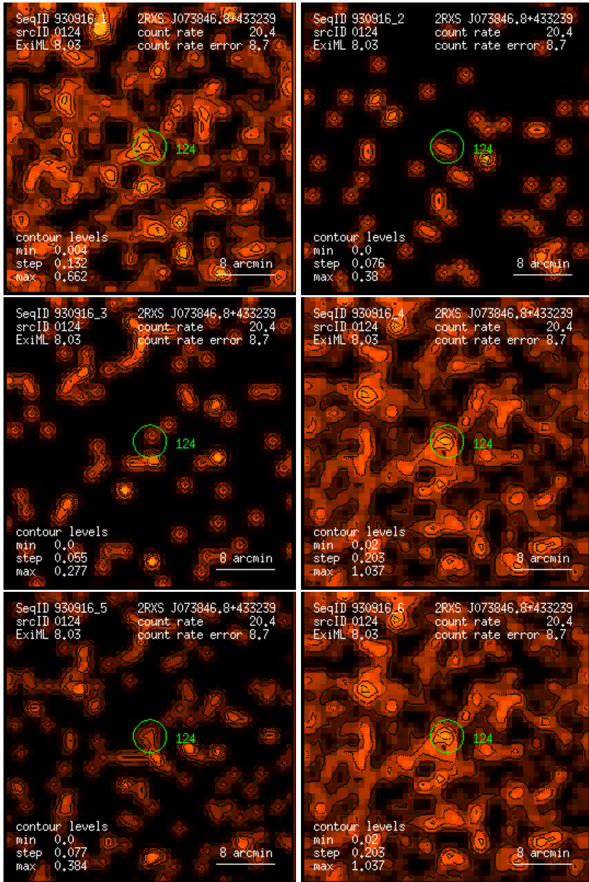
Figure 124: RASS 930916: detection 0124: band rate images, Gaussian filter: (1) PSPC channels 11 – 41, (2) 52 – 90, (3) 91 – 201, (4) 11 – 235, (5) 52 – 201, (6) 11 – 201. Broad band rates in counts/ks. Band rate contour levels in counts/ks/arcmin 2 .
