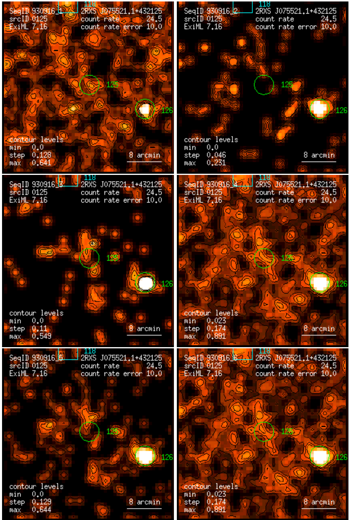
Figure 125: RASS 930916: detection 0125: band rate images, Gaussian filter: (1) PSPC channels 11 – 41, (2) 52 – 90, (3) 91 – 201, (4) 11 – 235, (5) 52 – 201, (6) 11 – 201. Broad band rates in counts/ks. Band rate contour levels in counts/ks/arcmin 2 .
