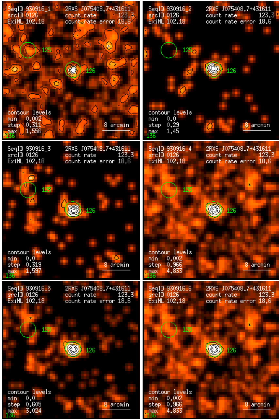
Figure 126: RASS 930916: detection 0126: band rate images, Gaussian filter: (1) PSPC channels 11 – 41, (2) 52 – 90, (3) 91 – 201, (4) 11 – 235, (5) 52 – 201, (6) 11 – 201. Broad band rates in counts/ks. Band rate contour levels in counts/ks/arcmin 2 .
