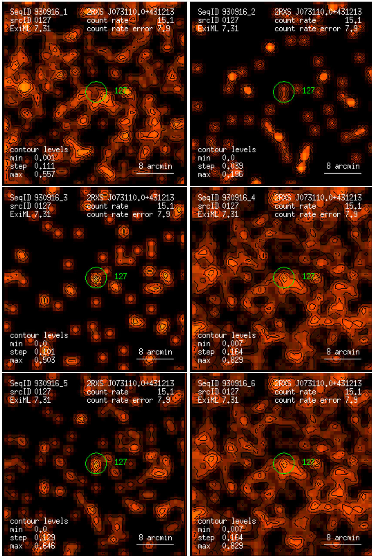
Figure 127: RASS 930916: detection 0127: band rate images, Gaussian filter: (1) PSPC channels 11 – 41, (2) 52 – 90, (3) 91 – 201, (4) 11 – 235, (5) 52 – 201, (6) 11 – 201. Broad band rates in counts/ks. Band rate contour levels in counts/ks/arcmin 2 .
