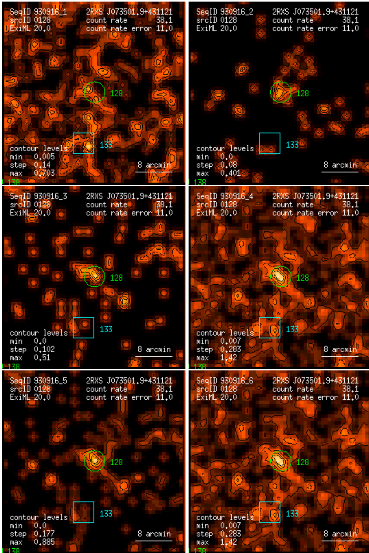
Figure 128: RASS 930916: detection 0128: band rate images, Gaussian filter: (1) PSPC channels 11 – 41, (2) 52 – 90, (3) 91 – 201, (4) 11 – 235, (5) 52 – 201, (6) 11 – 201. Broad band rates in counts/ks. Band rate contour levels in counts/ks/arcmin 2 .
