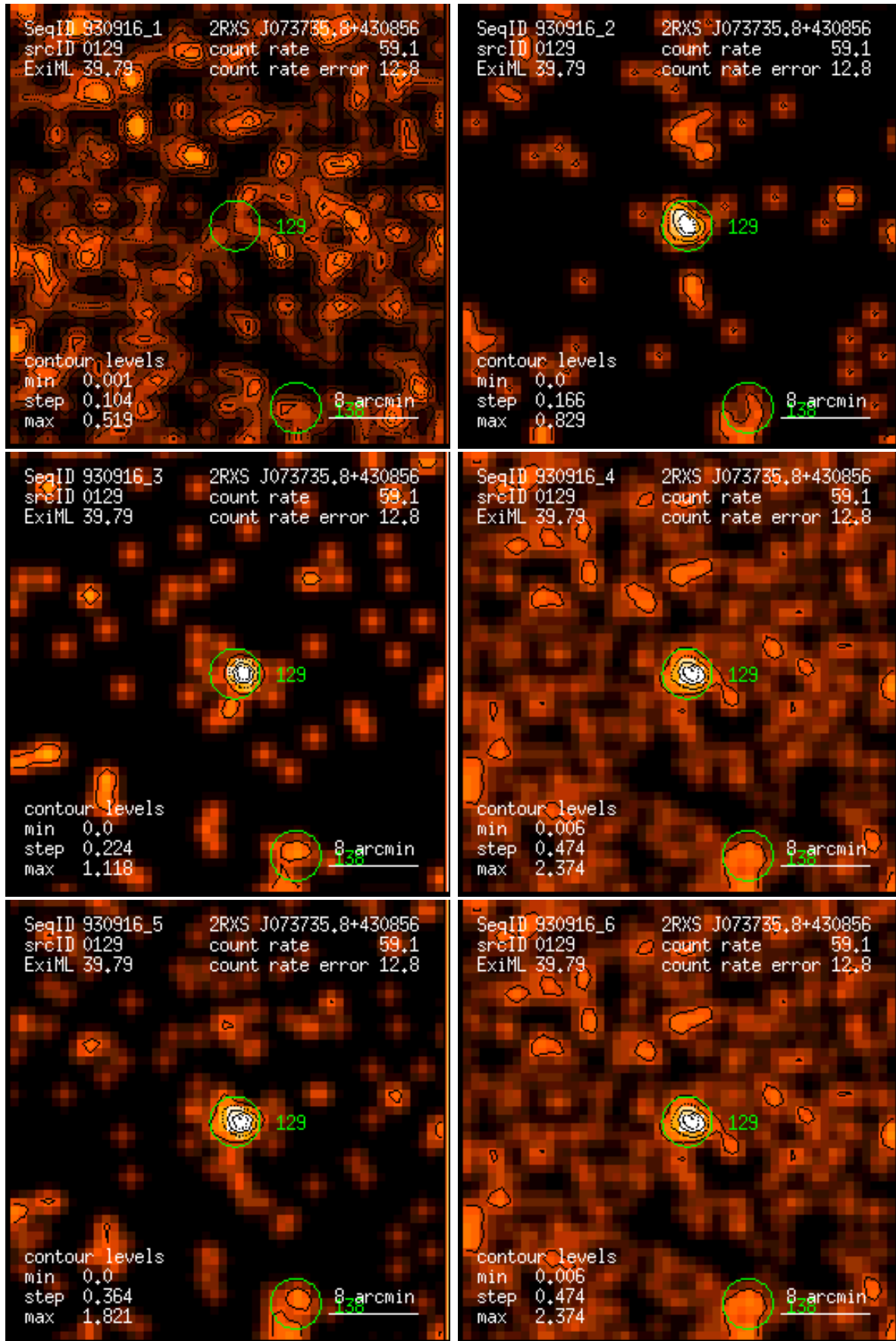
Figure 129: RASS 930916: detection 0129: band rate images, Gaussian filter: (1) PSPC channels 11 – 41, (2) 52 – 90, (3) 91 – 201, (4) 11 – 235, (5) 52 – 201, (6) 11 – 201. Broad band rates in counts/ks. Band rate contour levels in counts/ks/arcmin 2 .
