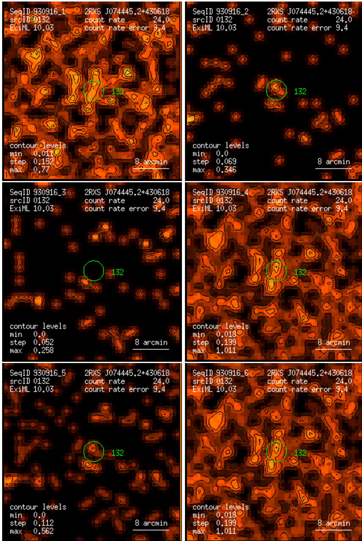
Figure 132: RASS 930916: detection 0132: band rate images, Gaussian filter: (1) PSPC channels 11 – 41, (2) 52 – 90, (3) 91 – 201, (4) 11 – 235, (5) 52 – 201, (6) 11 – 201. Broad band rates in counts/ks. Band rate contour levels in counts/ks/arcmin 2 .
