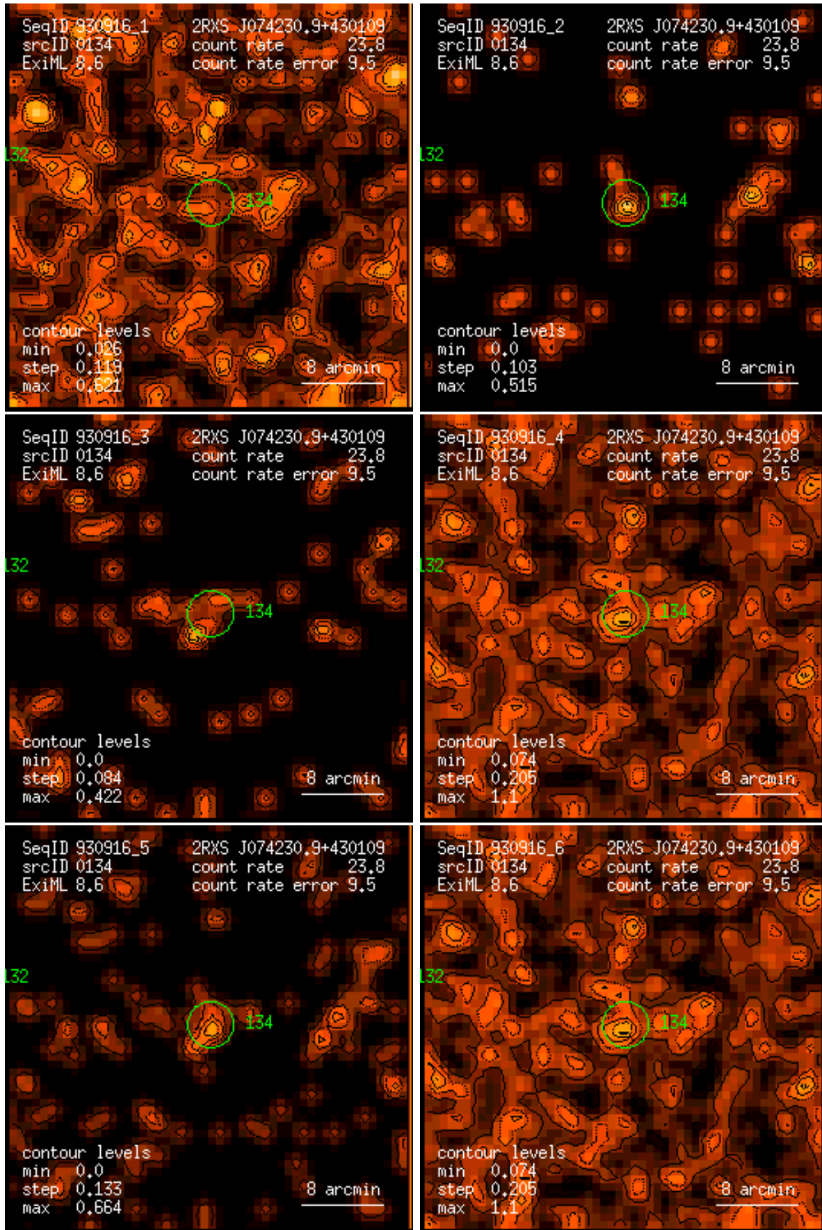
Figure 134: RASS 930916: detection 0134: band rate images, Gaussian filter: (1) PSPC channels 11 – 41, (2) 52 – 90, (3) 91 – 201, (4) 11 – 235, (5) 52 – 201, (6) 11 – 201. Broad band rates in counts/ks. Band rate contour levels in counts/ks/arcmin 2 .
