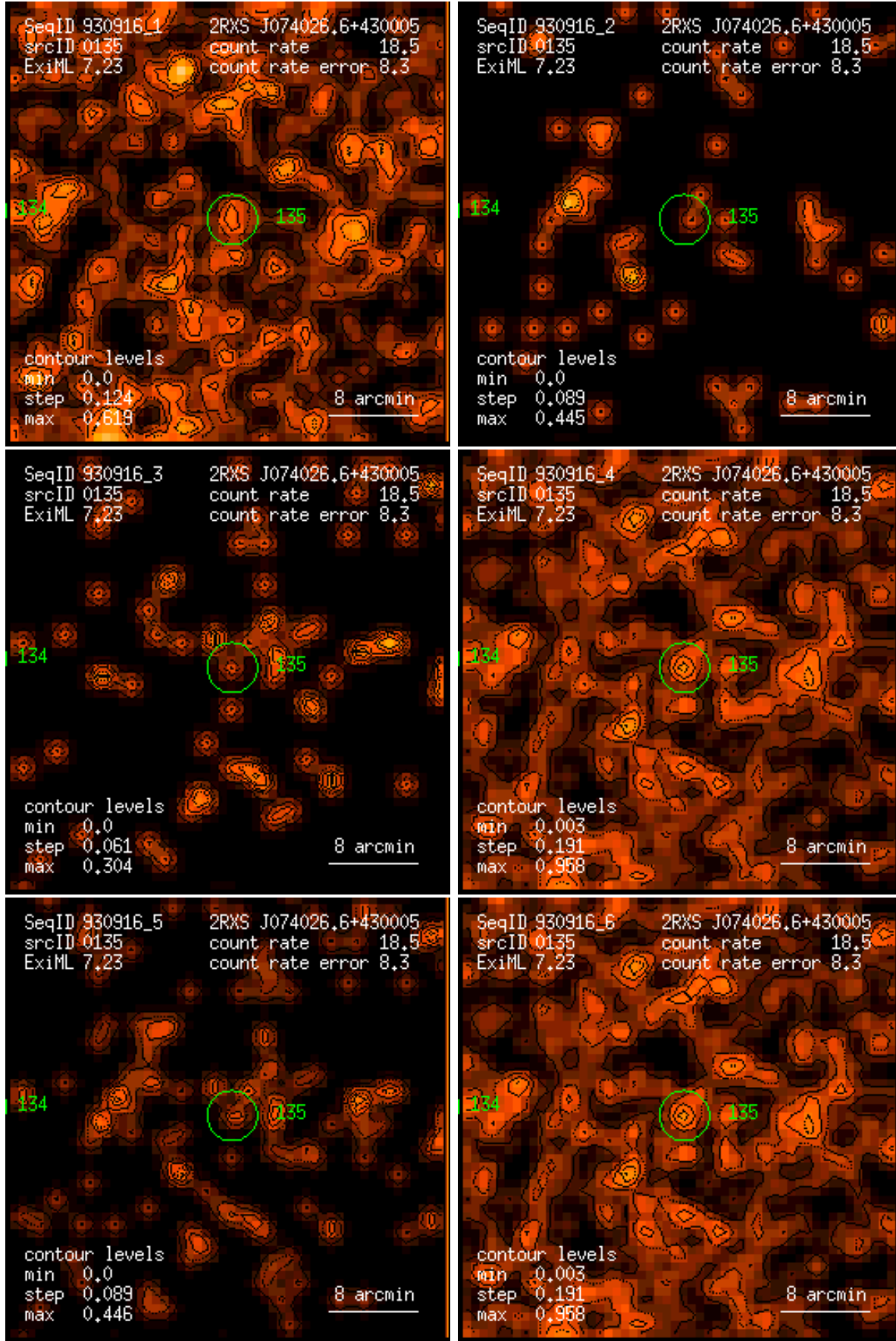
Figure 135: RASS 930916: detection 0135: band rate images, Gaussian filter: (1) PSPC channels 11 – 41, (2) 52 – 90, (3) 91 – 201, (4) 11 – 235, (5) 52 – 201, (6) 11 – 201. Broad band rates in counts/ks. Band rate contour levels in counts/ks/arcmin 2 .
