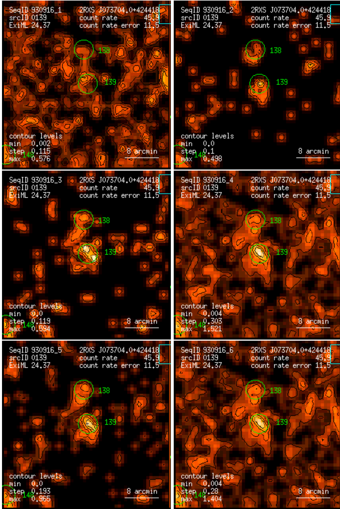
Figure 139: RASS 930916: detection 0139: band rate images, Gaussian filter: (1) PSPC channels 11 – 41, (2) 52 – 90, (3) 91 – 201, (4) 11 – 235, (5) 52 – 201, (6) 11 – 201. Broad band rates in counts/ks. Band rate contour levels in counts/ks/arcmin 2 .
