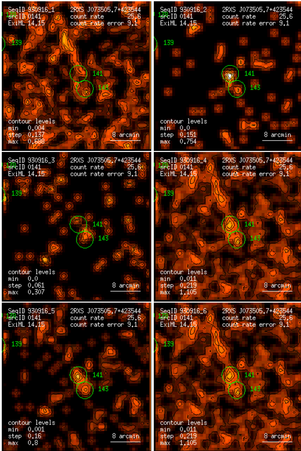
Figure 141: RASS 930916: detection 0141: band rate images, Gaussian filter: (1) PSPC channels 11 – 41, (2) 52 – 90, (3) 91 – 201, (4) 11 – 235, (5) 52 – 201, (6) 11 – 201. Broad band rates in counts/ks. Band rate contour levels in counts/ks/arcmin 2 .
