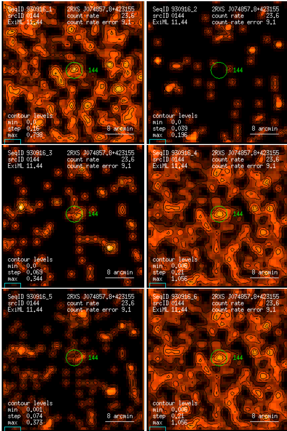
Figure 144: RASS 930916: detection 0144: band rate images, Gaussian filter: (1) PSPC channels 11 – 41, (2) 52 – 90, (3) 91 – 201, (4) 11 – 235, (5) 52 – 201, (6) 11 – 201. Broad band rates in counts/ks. Band rate contour levels in counts/ks/arcmin 2 .
