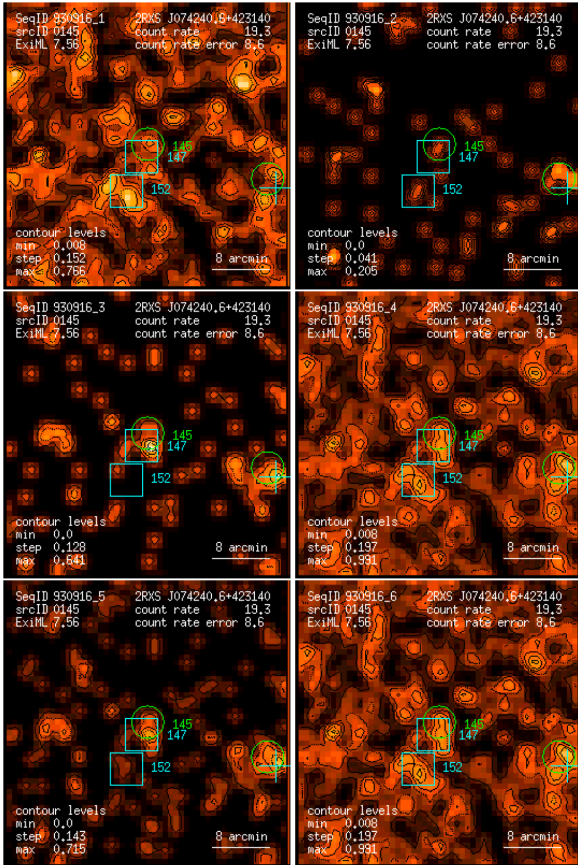
Figure 145: RASS 930916: detection 0145: band rate images, Gaussian filter: (1) PSPC channels 11 – 41, (2) 52 – 90, (3) 91 – 201, (4) 11 – 235, (5) 52 – 201, (6) 11 – 201. Broad band rates in counts/ks. Band rate contour levels in counts/ks/arcmin 2 .
