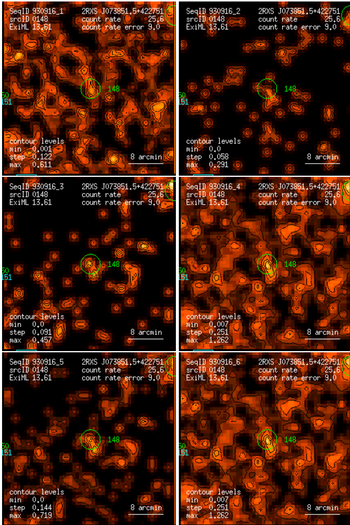
Figure 148: RASS 930916: detection 0148: band rate images, Gaussian filter: (1) PSPC channels 11 – 41, (2) 52 – 90, (3) 91 – 201, (4) 11 – 235, (5) 52 – 201, (6) 11 – 201. Broad band rates in counts/ks. Band rate contour levels in counts/ks/arcmin 2 .
