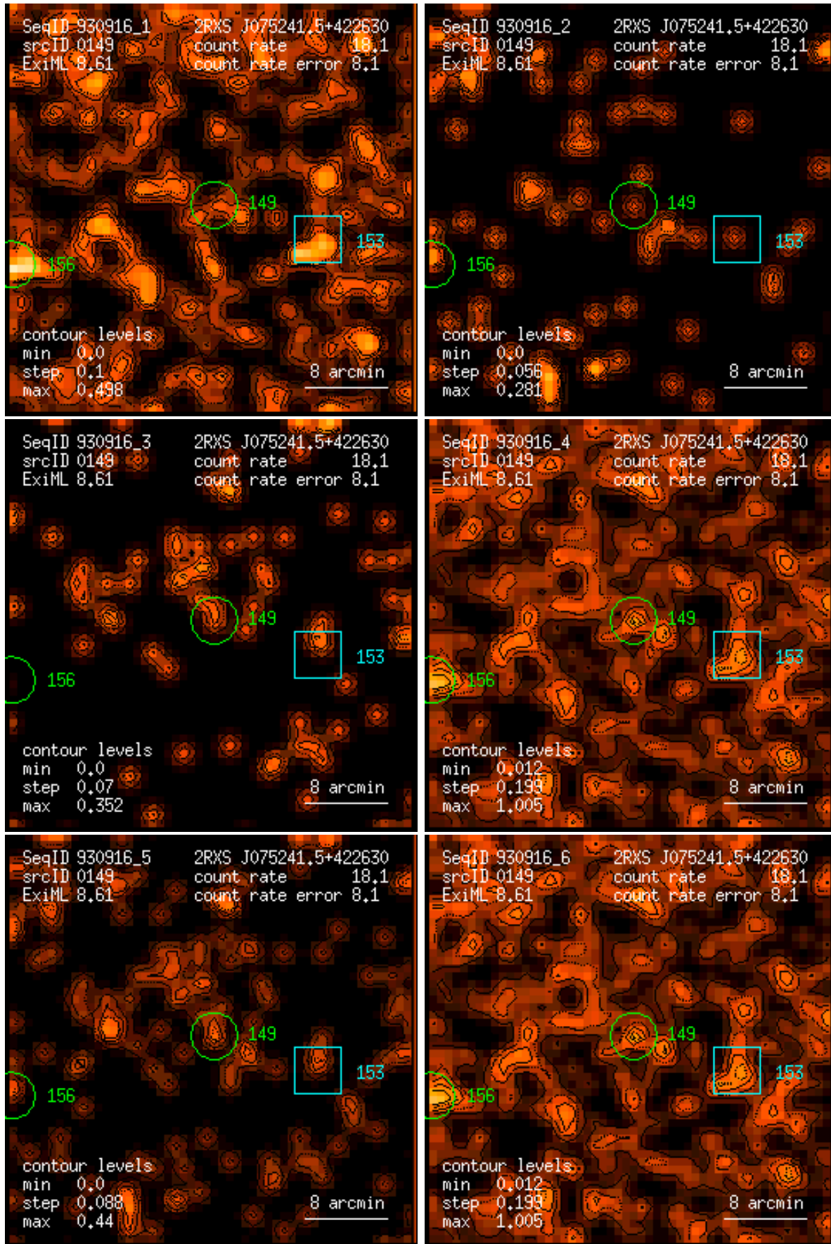
Figure 149: RASS 930916: detection 0149: band rate images, Gaussian filter: (1) PSPC channels 11 – 41, (2) 52 – 90, (3) 91 – 201, (4) 11 – 235, (5) 52 – 201, (6) 11 – 201. Broad band rates in counts/ks. Band rate contour levels in counts/ks/arcmin 2 .
