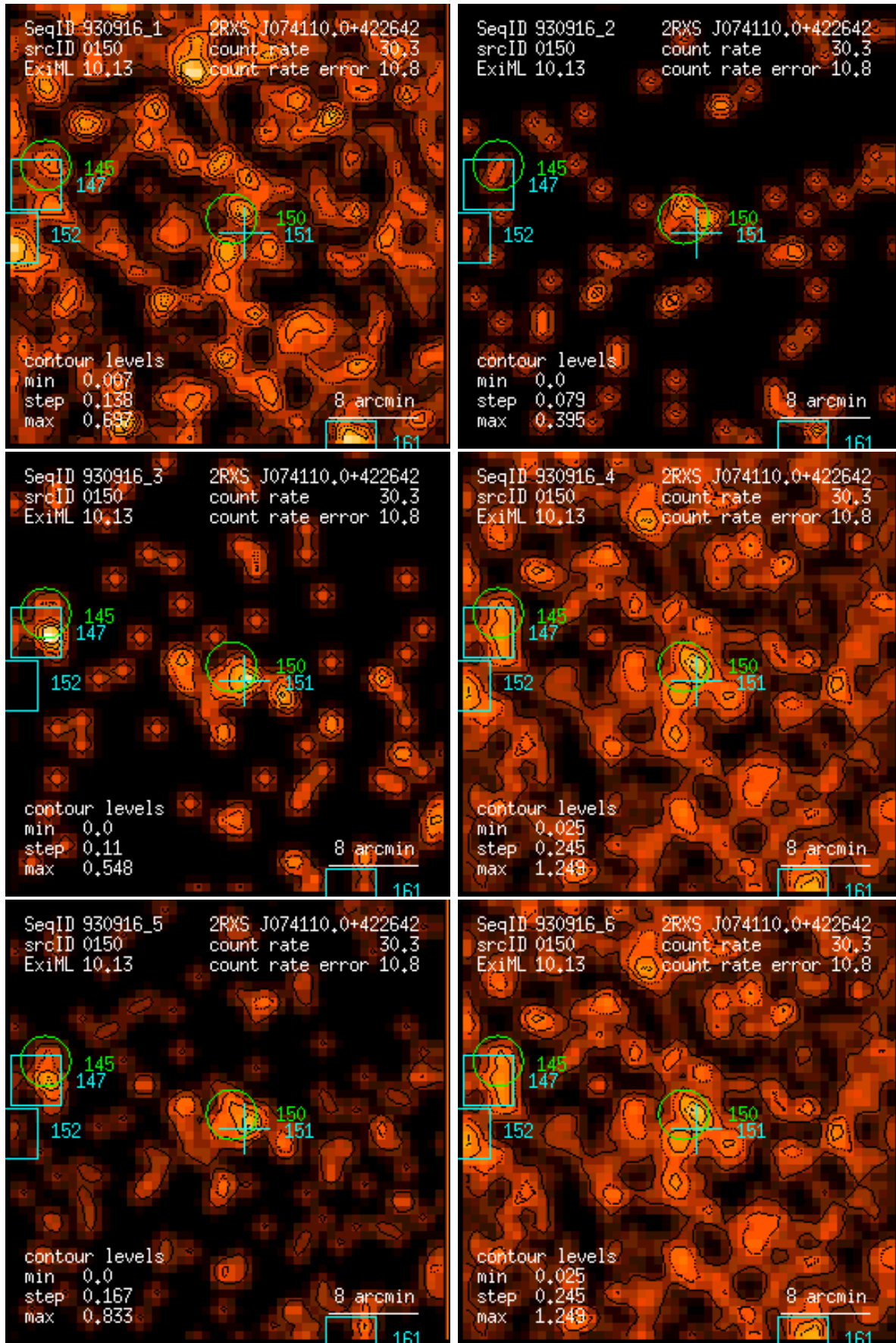
Figure 150: RASS 930916: detection 0150: band rate images, Gaussian filter: (1) PSPC channels 11 – 41, (2) 52 – 90, (3) 91 – 201, (4) 11 – 235, (5) 52 – 201, (6) 11 – 201. Broad band rates in counts/ks. Band rate contour levels in counts/ks/arcmin 2 .
